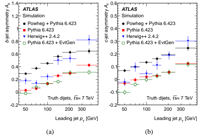
Fig. 3 The asymmetries in the amount of (a) bottom and (b) charm truth particle jets as taken from POWHEG+PYTHIA 6.423 (black points), PYTHIA 6.423 (squares), Herwig++ 2.4.2 (triangles) and PYTHIA+EVTGEN (open squares) in leading and subleading jets, for each leading jet p_T bin used in the analysis.
