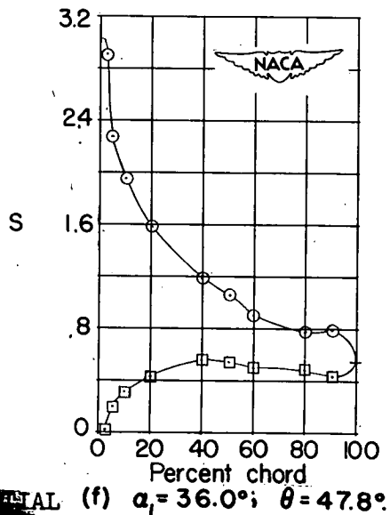
Figure 44.- Blade-surface pressure distributions and blade section characteristics for the cascade combination, \beta_1 = 45^\circ , \sigma = 1.50 , and blade section, NACA 65-(18)10.
