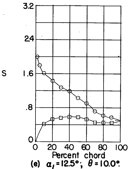
Figure 72.- Blade-surface pressure distributions and blade section characteristics for the cascade combination, \beta_1 = 70^\circ , \sigma = 1.00 , and blade section, NACA 65-410.
