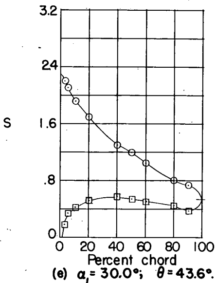
Figure 44.- Blade-surface pressure distributions and blade section characteristics for the cascade combination, \beta_1 = 45^\circ , \sigma = 1.50 , and blade section, NACA 65-(18)10.
