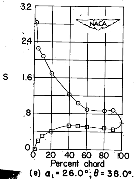
Figure 38.- Blade-surface pressure distributions and blade section characteristics for the cascade combination, \beta_1 = 45^\circ , \sigma = 1.25 , and blade section, NACA 65-(18)10.
