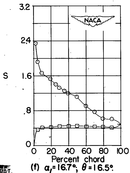
Figure 55.- Blade-surface pressure distributions and blade section characteristics for the cascade combination, \beta_1 = 60^\circ , \sigma = 1.00 , and blade section, NACA 65-810.
