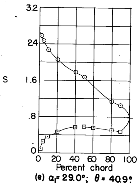
Figure 11.- Blade-surface pressure distributions and blade section characteristics for the cascade combination, \beta_1 = 30^\circ , \sigma = 1.00 , and blade section, NACA 65-(18)10.
