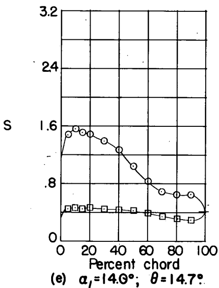
Figure 75.- Blade-surface pressure distributions and blade section characteristics for the cascade combination, \beta_1 = 70^\circ , \sigma = 1.00 , and blade section, NACA 65-(15)10.
