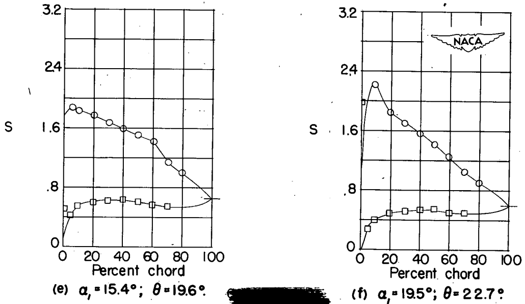
Figure 25.- Blade-surface pressure distributions and blade section characteristics for the cascade combination, \beta_1 = 45^\circ , \sigma = 0.75 , and blade section, NACA 65-(12)10
