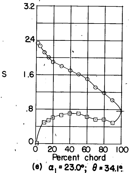
Figure 10.- Blade-surface pressure distributions and blade section characteristics for the cascade combination, \beta_1 = 30^\circ , \sigma = 1.00 , and blade section, NACA 65-(15)10.
