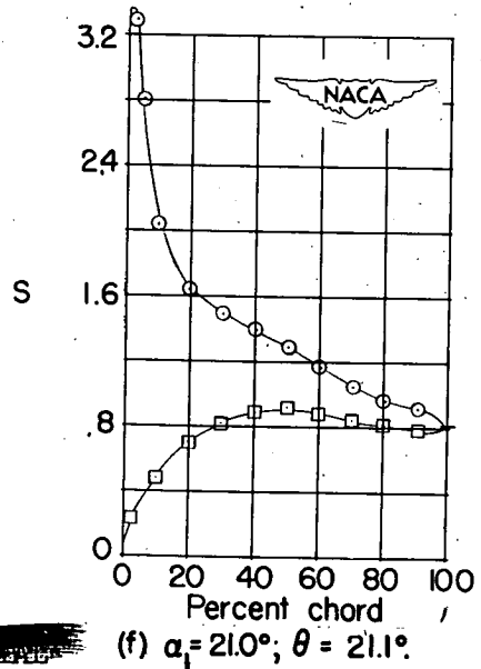
Figure 7.- Blade-surface pressure distributions and blade section characteristics for the cascade combination, \beta_1 = 30^\circ , \sigma = 1.00 , and blade section, NACA 65-410.
