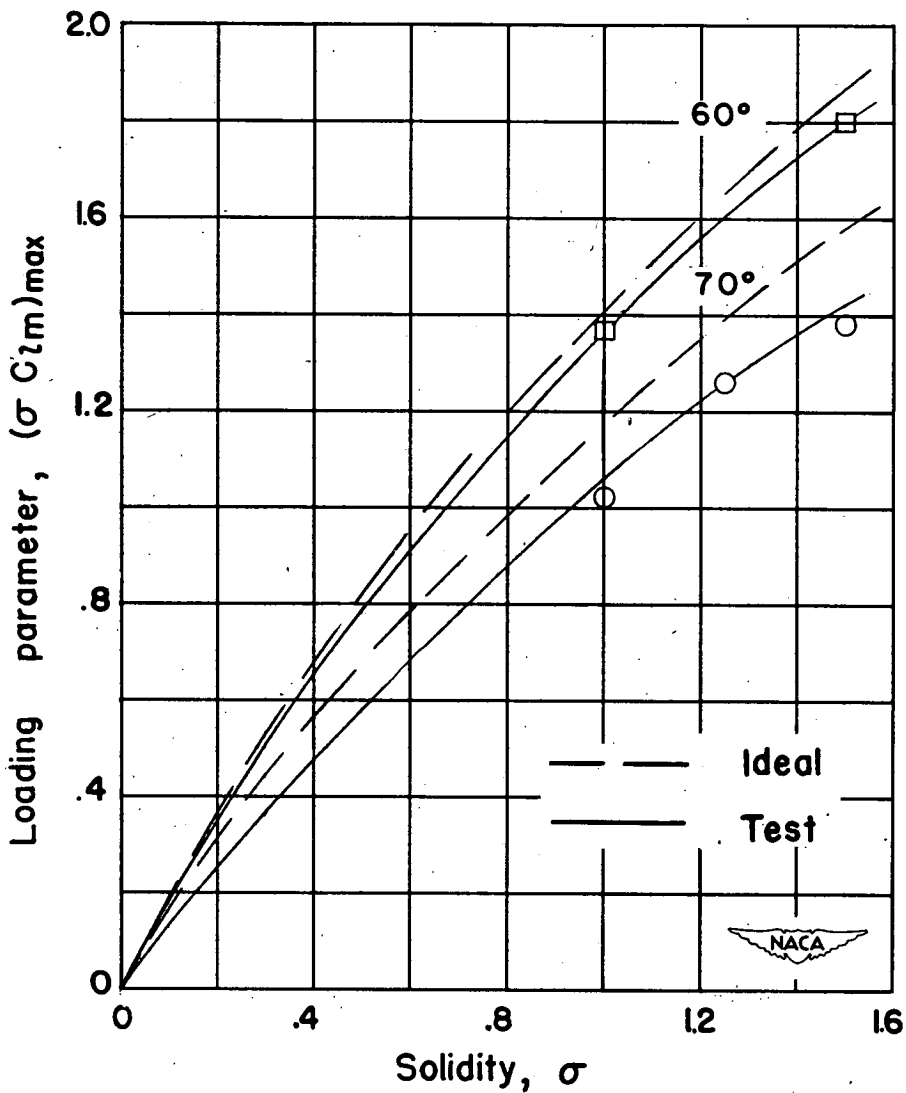
Figure 89.- Variation of the limit loading parameter, (\sigma C_{lm})_{max} with solidity for inlet angles of 60° and 70°.
