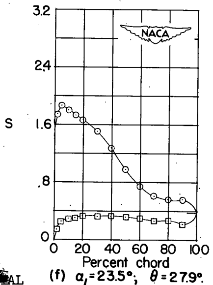
Figure 59.- Blade-surface pressure distributions and blade section characteristics for the cascade combination, \beta_1 = 60^\circ , \sigma = 1.00 , and blade section, NACA 65-(21)10.
