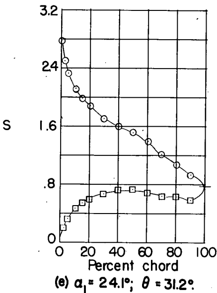
Figure 9.- Blade-surface pressure distributions and blade section characteristics for the cascade combination, \beta_1 = 30^\circ , \sigma = 1.00 , and blade section, NACA 65-(12)10.
