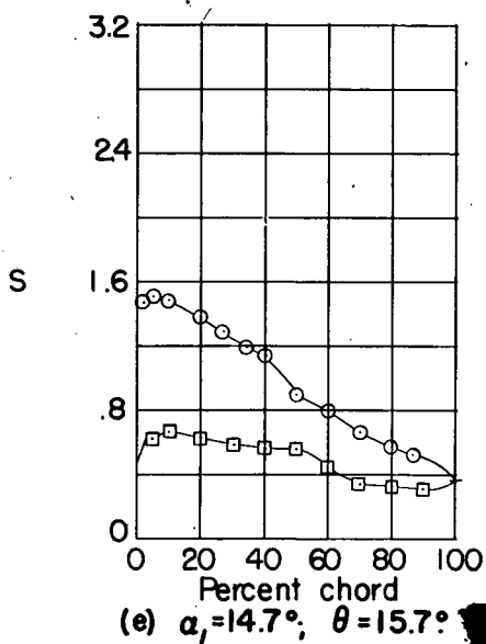
Figure 82.- Blade-surface pressure distributions and blade section characteristics for the cascade combination, \beta_1 = 70^\circ , \sigma = 1.50 , and blade section, NACA 65-810.
