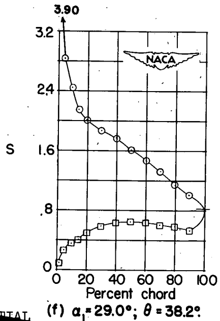
Figure 10.- Blade-surface pressure distributions and blade section characteristics for the cascade combination, \beta_1 = 30^\circ , \sigma = 1.00 , and blade section, NACA 65-(15)10.
