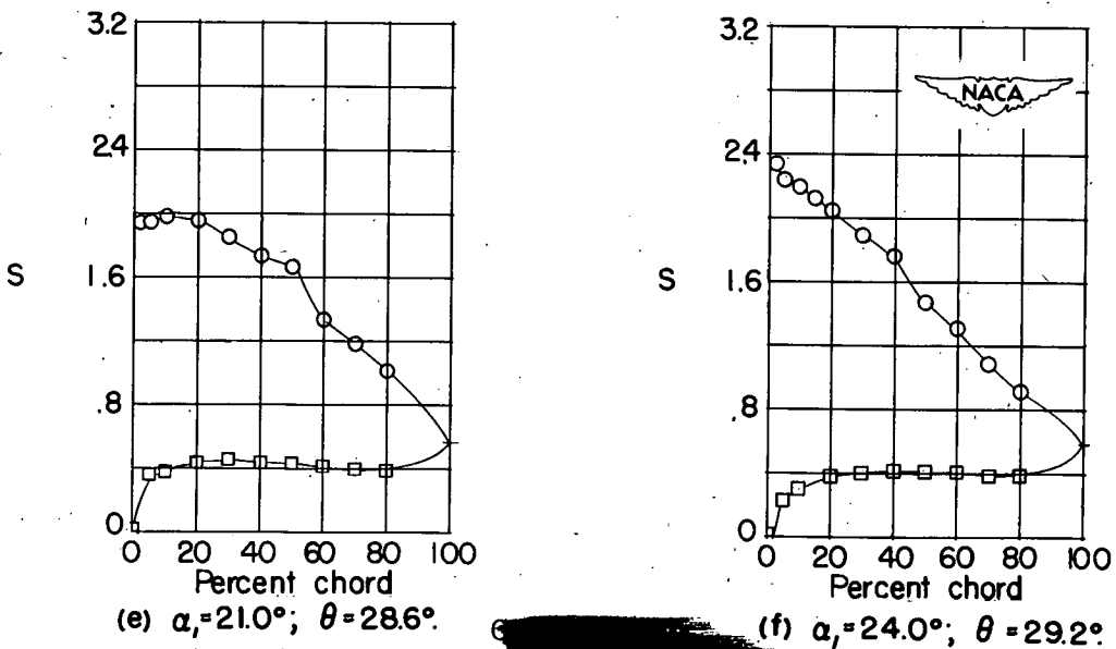
Figure 26.- Blade-surface pressure distributions and blade section characteristics for the cascade combination, \beta_1 = 45^\circ , \sigma = 0.75 , and blade section, NACA 65-(18)10.
