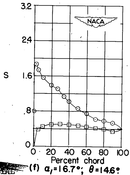
Figure 77.- Blade-surface pressure distributions and blade section characteristics for the cascade combination, \beta_1 = 70^\circ , \sigma = 1.25 , and blade section, NACA 65-810.
