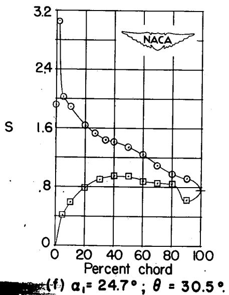
Figure 17.- Blade-surface pressure distributions and blade section characteristics for the cascade combination, \beta_1 = 30^\circ , \sigma = 1.50 , and blade section, NACA 65-810.
