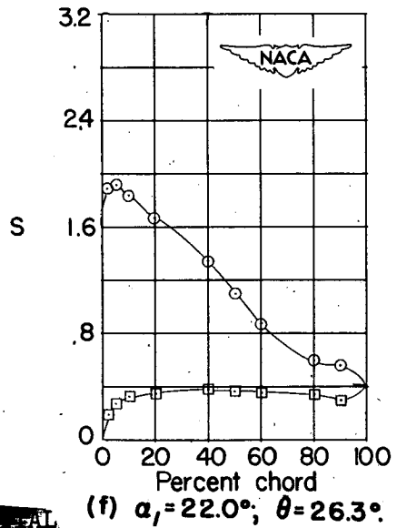
Figure 58.- Blade-surface pressure distributions and blade section characteristics for the cascade combination, \beta_1 = 60^\circ , \sigma = 1.00 , and blade section, NACA 65-(18)10.
