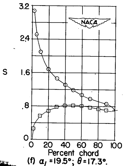
Figure 28.- Blade-surface pressure distributions and blade section characteristics for the cascade combination, \beta_1 = 45^\circ , \sigma = 1.00 , and blade section, NACA 65-410.
