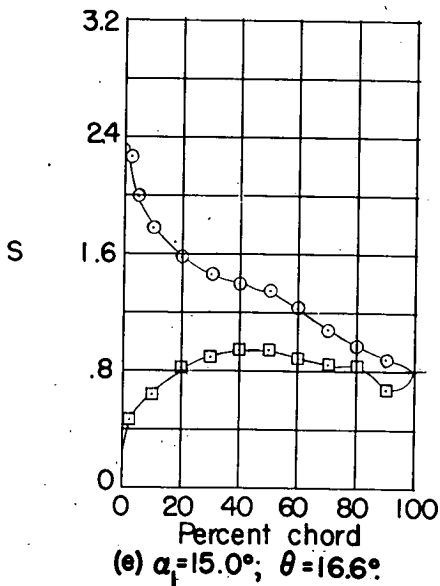
Figure 7.- Blade-surface pressure distributions and blade section characteristics for the cascade combination, \beta_1 = 30^\circ , \sigma = 1.00 , and blade section, NACA 65-410.
