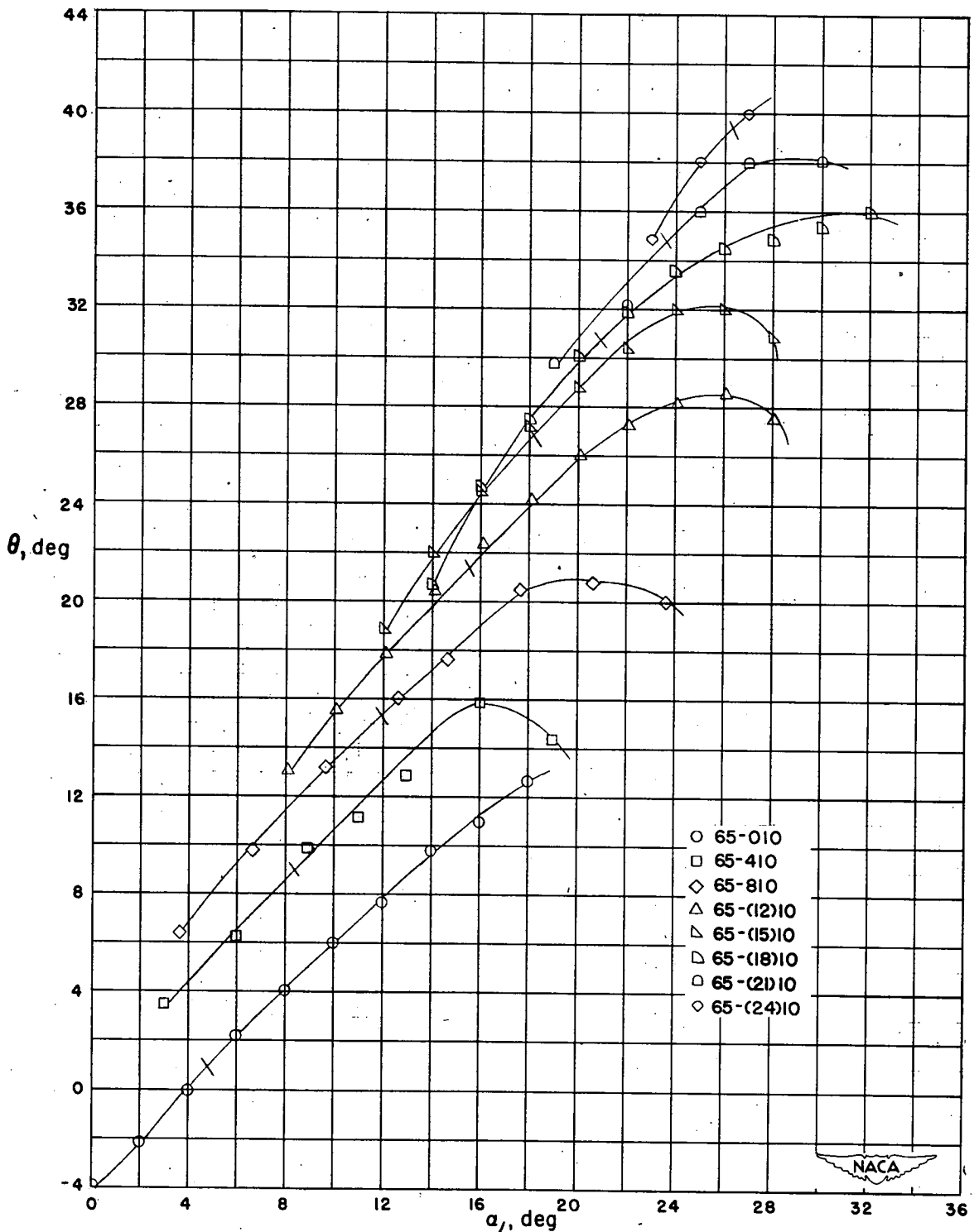
Figure 103.- Summary of turning angle, \theta , angle of attack, \alpha , relationship for the blade sections tested at \beta_1 = 60^\circ , \sigma = 1.50 . Short bars across curves indicate design points.
