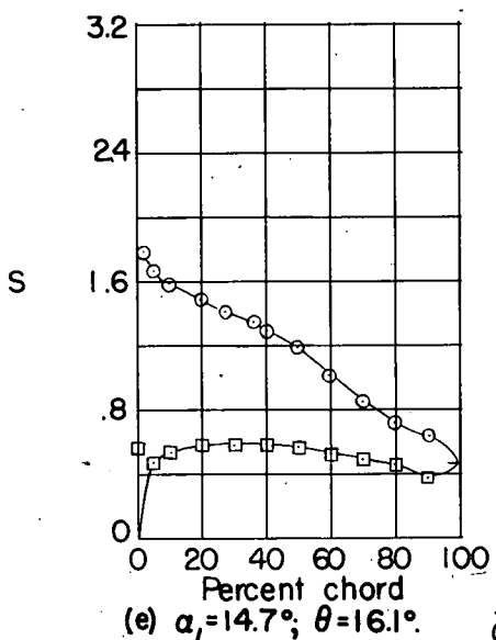
Figure 55.- Blade-surface pressure distributions and blade section characteristics for the cascade combination, \beta_1 = 60^\circ , \sigma = 1.00 , and blade section, NACA 65-810.
