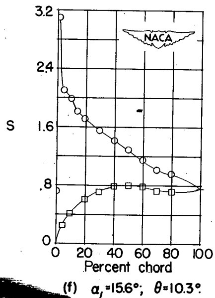
Figure 21.- Blade-surface pressure distributions and blade section characteristics for the cascade combination, \beta_1 = 45^\circ , \sigma = 0.50 , and blade section, NACA 65-410.
