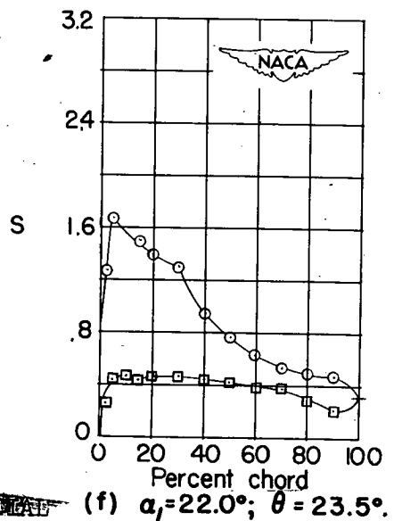
Figure 84.- Blade-surface pressure distributions and blade section characteristics for the cascade combination, \beta_1 = 70^\circ , \sigma = 1.50 , and blade section, NACA 65-(15)10.
