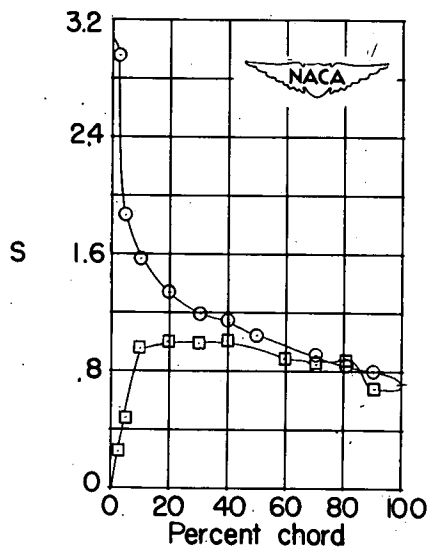
(f) \alpha_1 = 17.0^\circ; \theta = 14.7^\circ .
