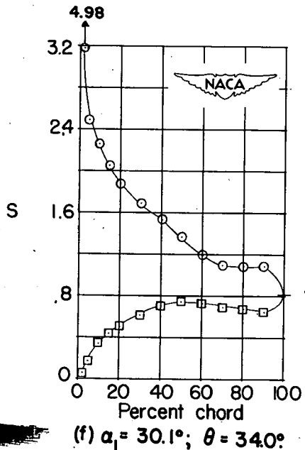
Figure 9.- Blade-surface pressure distributions and blade section characteristics for the cascade combination, \beta_1 = 30^\circ , \sigma = 1.00 , and blade section, NACA 65-(12)10.
