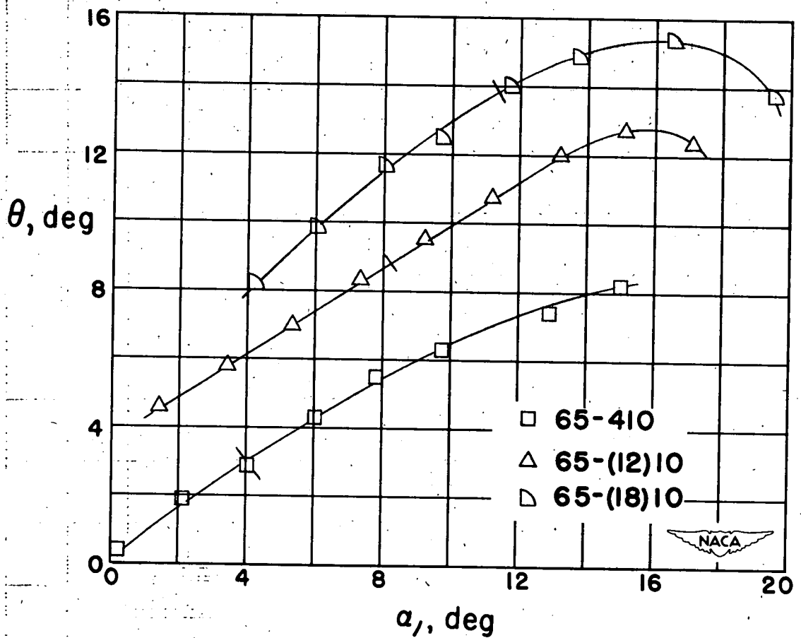
Figure 99.- Summary of turning angle, \theta , angle of attack, \alpha , relationship for the blade sections tested at \beta_1 = 60^\circ , \sigma = 0.50 . Short vertical bars across curves indicate design points.
