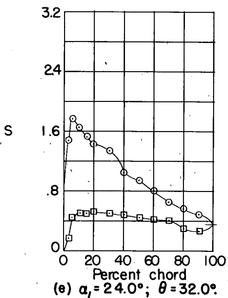
Figure 67.- Blade-surface pressure distributions and blade section characteristics for the cascade combination, \beta_1 = 60^\circ , \sigma = 1.50 , and blade section, NACA 65-(15)10.
