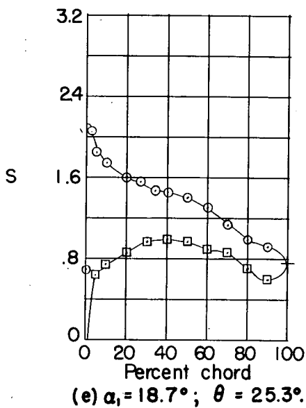
Figure 17.- Blade-surface pressure distributions and blade section characteristics for the cascade combination, \beta_1 = 30^\circ , \sigma = 1.50 , and blade section, NACA 65-810.
