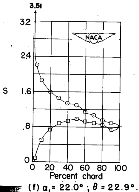
Figure 12.- Blade-surface pressure distributions and blade section characteristics for the cascade combination, \beta_1 = 30^\circ , \sigma = 1.25 , and blade section, NACA 65-410.
