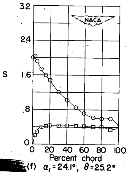
Figure 61.- Blade-surface pressure distributions and blade section characteristics for the cascade combination, \beta_1 = 60^\circ , \sigma = 1.25 , and blade section, NACA 65-(12)10.
