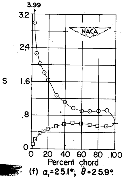
Figure 30.- Blade-surface pressure distributions and blade section characteristics for the cascade combination, \beta_1 = 45^\circ , \sigma = 1.00 , and blade section, NACA 65-(12)10.
