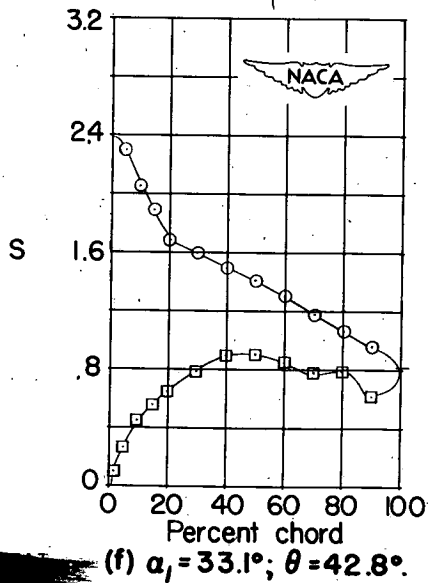
Figure 18.- Blade-surface pressure distributions and blade section characteristics for the cascade combination, \beta_1 = 30^\circ , \sigma = 1.50 , and blade section, NACA 65-(12)10.
