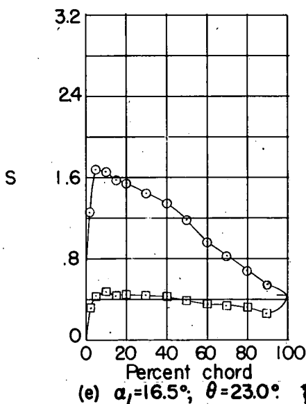
Figure 57.- Blade-surface pressure distributions and blade section characteristics for the cascade combination, \beta_1 = 60^\circ , \sigma = 1.00 , and blade section, NACA 65-(15)10.
