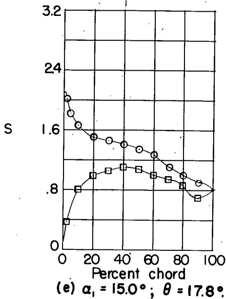
Figure 16.- Blade-surface pressure distributions and blade section characteristics for the cascade combination, \beta_1 = 30^\circ , \sigma = 1.50 , and blade section, NACA 65-410.
