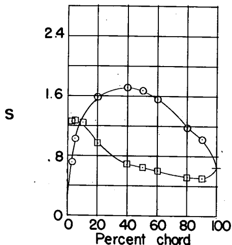
(a) \alpha_1 = 9.0^\circ ; \theta = 17.9^\circ
