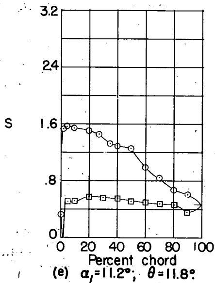
Figure 73.- Blade-surface pressure distributions and blade section characteristics for the cascade combination, \beta_1 = 70^\circ , \sigma = 1.00 , and blade section, NACA 65-810.
