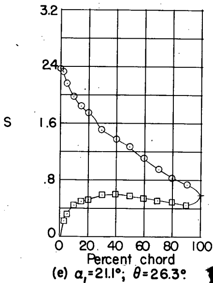
Figure 30.- Blade-surface pressure distributions and blade section characteristics for the cascade combination, \beta_1 = 45^\circ , \sigma = 1.00 , and blade section, NACA 65-(12)10.
