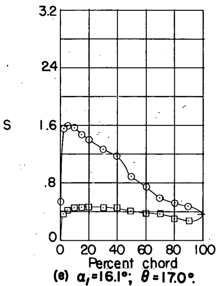
Figure 78.- Blade-surface pressure distributions and blade section characteristics for the cascade combination, \beta_1 = 70^\circ , \sigma = 1.25 , and blade section, NACA 65-(12)10.
