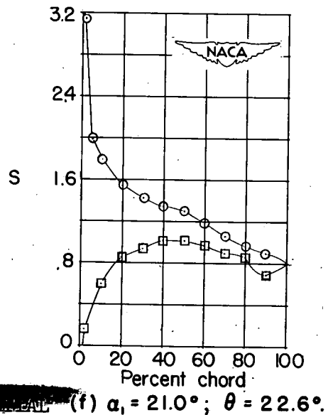
Figure 16.- Blade-surface pressure distributions and blade section characteristics for the cascade combination, \beta_1 = 30^\circ , \sigma = 1.50 , and blade section, NACA 65-410.
