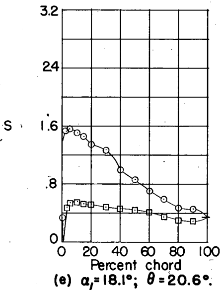
Figure 83.- Blade-surface pressure distributions and blade section characteristics for the cascade combination, \beta_1 = 70^\circ , \sigma = 1.50 , and blade section, NACA 65-(12)10.
