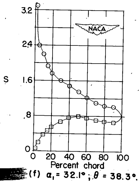
Figure 13.- Blade-surface pressure distributions and blade section characteristics for the cascade combination, \beta_1 = 30^\circ , \sigma = 1.25 , and blade section, NACA 65-(12)10.
