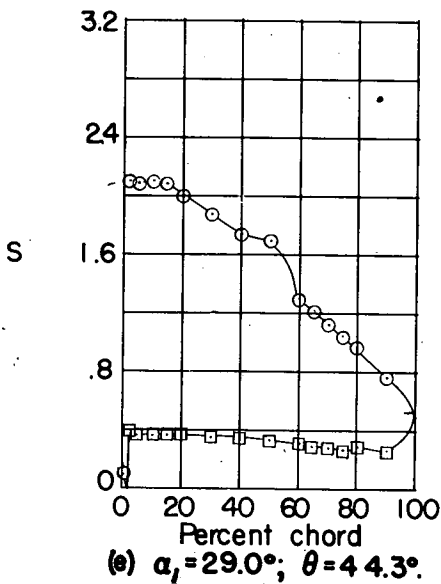
Figure 35.- Blade-surface pressure distributions and blade section characteristics for the cascade combination, \beta_1 = 45^\circ , \sigma = 1.00 and blade section, NACA 65-(27)10.
