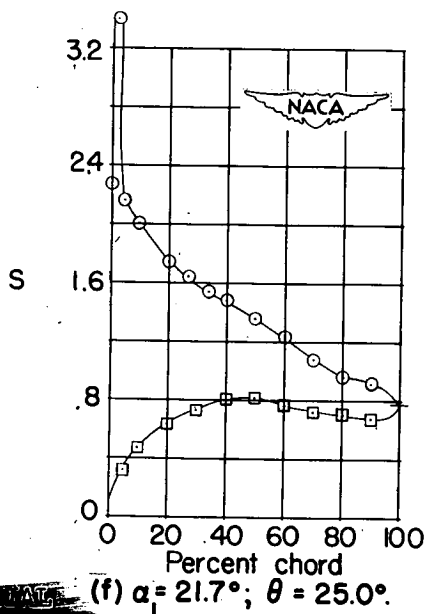
Figure 8.- Blade-surface pressure distributions and blade section characteristics for the cascade combination, \beta_1 = 30^\circ , \sigma = 1.00 , and blade section, NACA 65-810.
