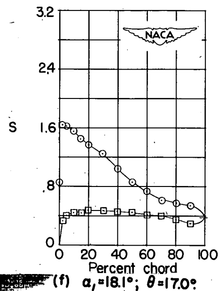
Figure 78.- Blade-surface pressure distributions and blade section characteristics for the cascade combination, \beta_1 = 70^\circ , \sigma = 1.25 , and blade section, NACA 65-(12)10.
