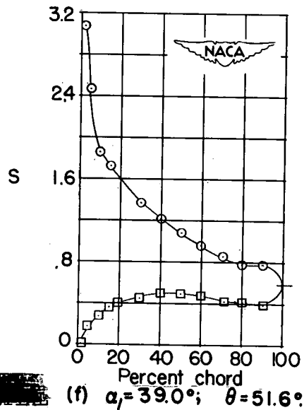
Figure 45.- Blade-surface pressure distributions and blade section characteristics for the cascade combination, \beta_1 = 45^\circ , \sigma = 1.50 , and blade section, NACA 65-(21)10.
