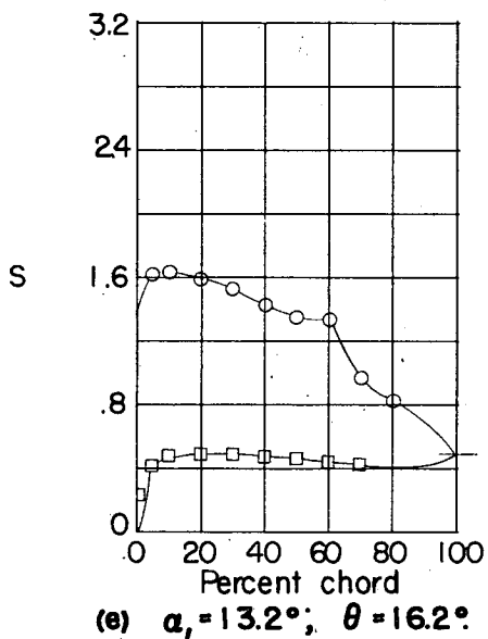
Figure 51.- Blade-surface pressure distributions and blade section characteristics for the cascade combination, \beta_1 = 60^\circ , \sigma = 0.75 , and blade section, NACA 65-(12)10.
