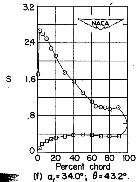
Figure 34.- Blade-surface pressure distributions and blade section characteristics for the cascade combination, \beta_1 = 45^\circ , \sigma = 1.00 , and blade section, NACA 65-(24)10.
