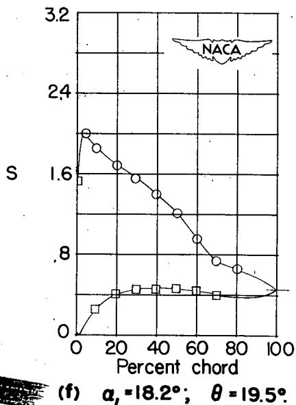
Figure 51.- Blade-surface pressure distributions and blade section characteristics for the cascade combination, \beta_1 = 60^\circ , \sigma = 0.75 , and blade section, NACA 65-(12)10.
