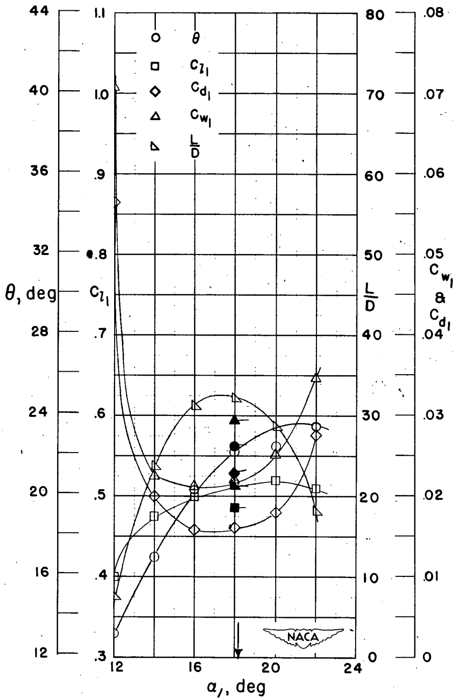
(g) Section characteristics; arrow shows design angle of attack; flagged symbol indicates leading-edge roughness; solid symbol indicates high Reynolds number.
