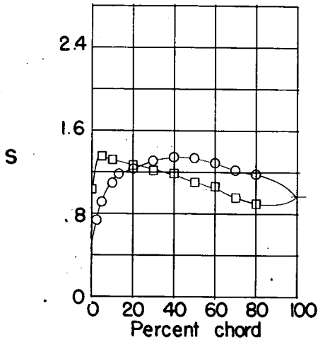
(a) \alpha_1 = 0.2^\circ ; \theta = 0.3^\circ
