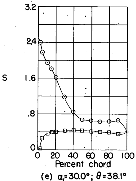
Figure 69.- Blade-surface pressure distributions and blade section characteristics for the cascade combination, \beta_1 = 60^\circ , \sigma = 1.50 , and blade section, NACA 65-(21)10.
