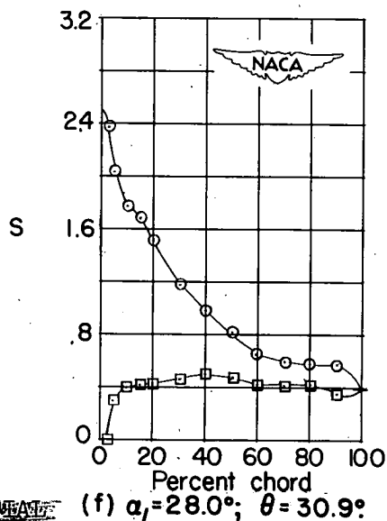
Figure 67.- Blade-surface pressure distributions and blade section characteristics for the cascade combination, \beta_1 = 60^\circ , \sigma = 1.50 , and blade section, NACA 65-(15)10.
