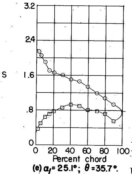
Figure 18.- Blade-surface pressure distributions and blade section characteristics for the cascade combination, \beta_1 = 30^\circ , \sigma = 1.50 , and blade section, NACA 65-(12)10.
