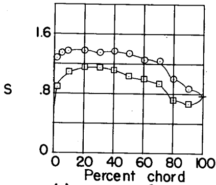
(c) \alpha_1 = 8.0^\circ ; \theta = 10.4^\circ
