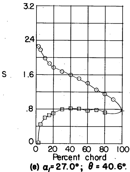
Figure 19.- Blade-surface pressure distributions and blade section characteristics for the cascade combination, \beta_1 = 30^\circ , \sigma = 1.50 , and blade section, NACA 65-(15)10.
