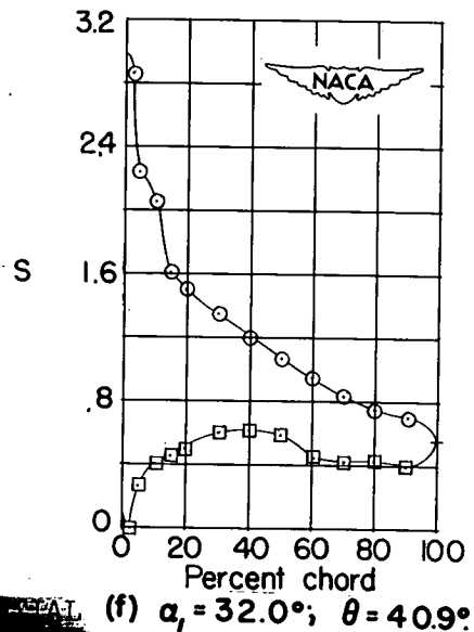
Figure 43.- Blade-surface pressure distributions and blade section characteristics for the cascade combination, \beta_1 = 45^\circ , \sigma = 1.50 , and blade section, NACA 65-(15)10.
