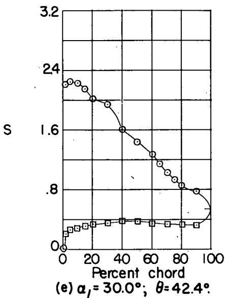
Figure 34.- Blade-surface pressure distributions and blade section characteristics for the cascade combination, \beta_1 = 45^\circ , \sigma = 1.00 , and blade section, NACA 65-(24)10.
