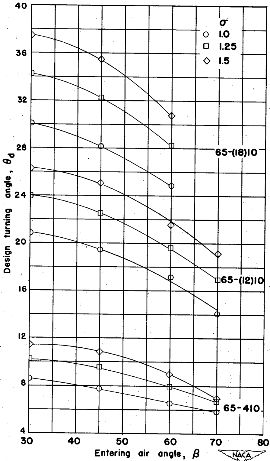
Figure 110.- Variation of design turning angle with inlet angle and solidity for typical sections.
