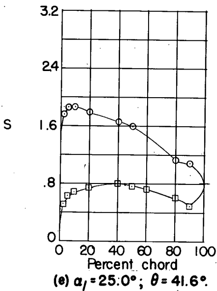
Figure 20.- Blade-surface pressure distributions and blade section characteristics for the cascade combination, \beta_1 = 30^\circ , \sigma = 1.50 , and blade section, NACA 65-(18)10.
