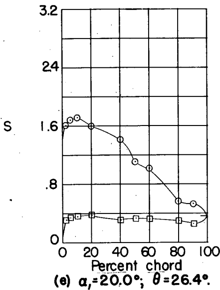
Figure 58.- Blade-surface pressure distributions and blade section characteristics for the cascade combination, \beta_1 = 60^\circ , \sigma = 1.00 , and blade section, NACA 65-(18)10.
