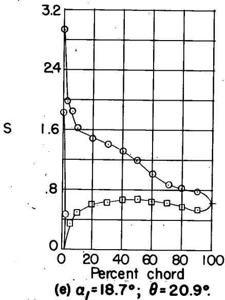
Figure 29.- Blade-surface pressure distributions and blade section characteristics for the cascade combination, \beta_1 = 45^\circ , \sigma = 1.00 , and blade section, NACA 65-810.
