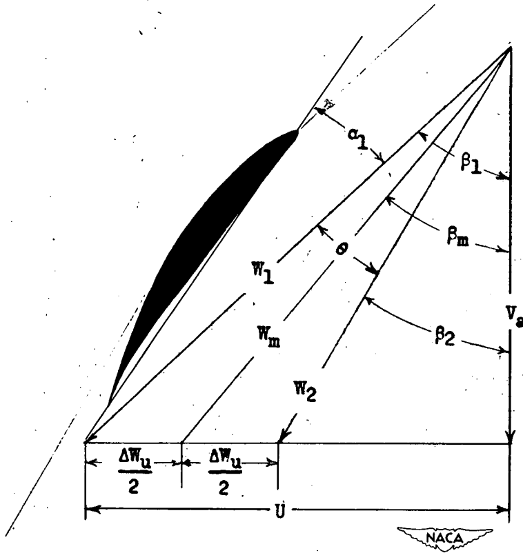
Figure 5.- Typical vector diagram for a compressor rotor.
