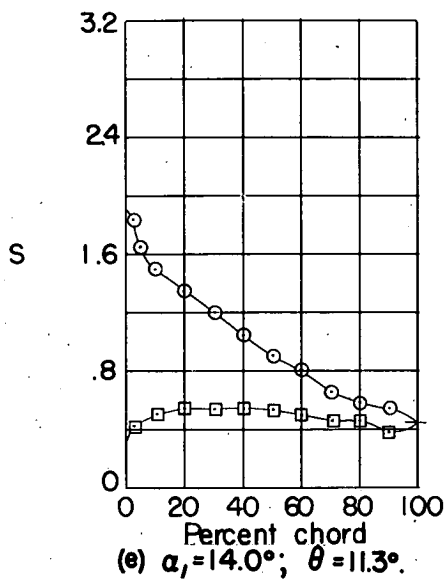
Figure 76.- Blade-surface pressure distributions and blade section characteristics for the cascade combination, \beta_1 = 70^\circ , \sigma = 1.25 , and blade section, NACA 65-410.
