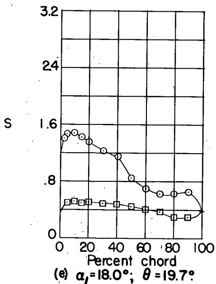
Figure 79.- Blade-surface pressure distributions and blade section characteristics for the cascade combination, \beta_1 = 70^\circ , \sigma = 1.25 , and blade section, NACA 65-(15)10.
