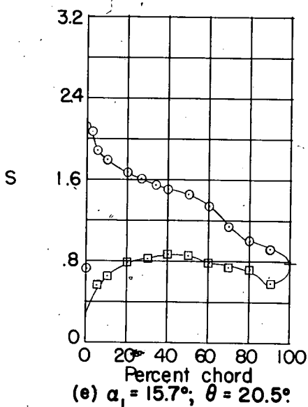
Figure 8.- Blade-surface pressure distributions and blade section characteristics for the cascade combination, \beta_1 = 30^\circ , \sigma = 1.00 , and blade section, NACA 65-810.
