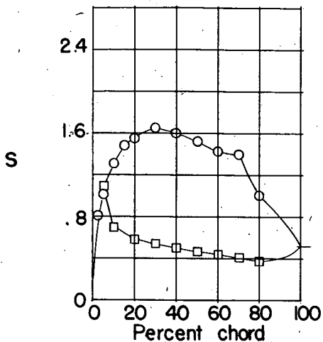
(a) \alpha_1 = 9.2^\circ ; \theta = 15.8^\circ
