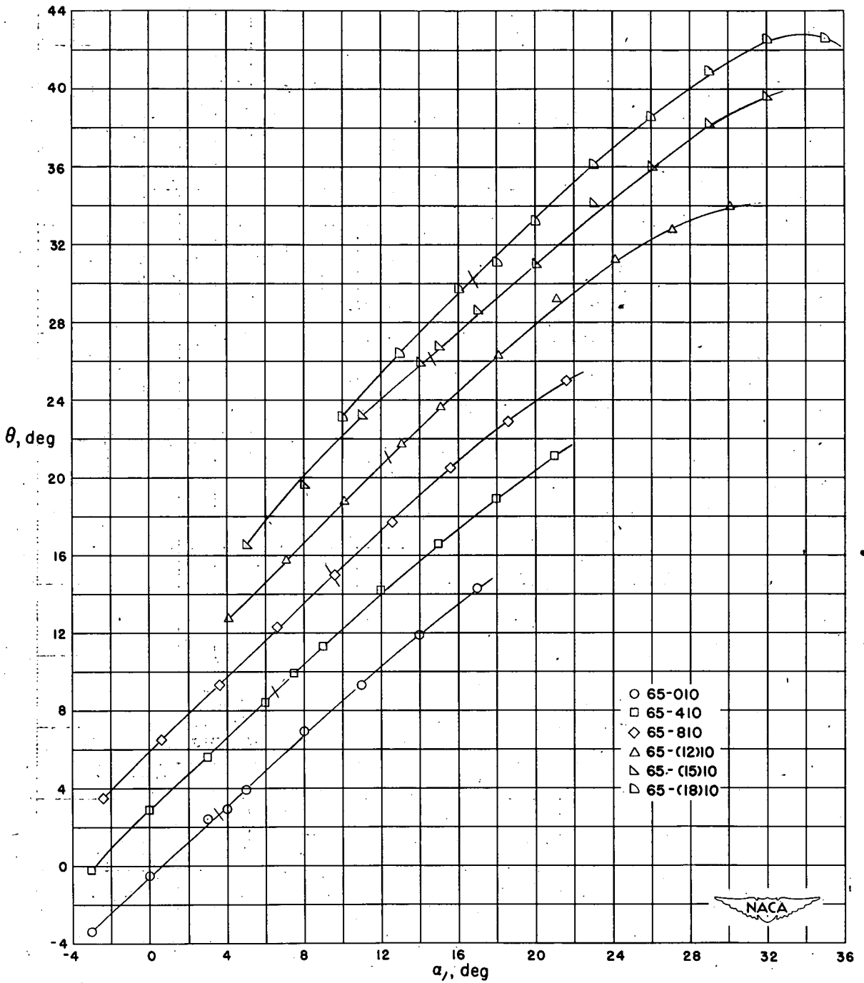
Figure 91.- Summary of turning angle, \theta , angle of attack, \alpha , relationship for the blade sections tested at \beta_1 = 30^\circ , \sigma = 1.00 . Short bars across curves indicate design points.
