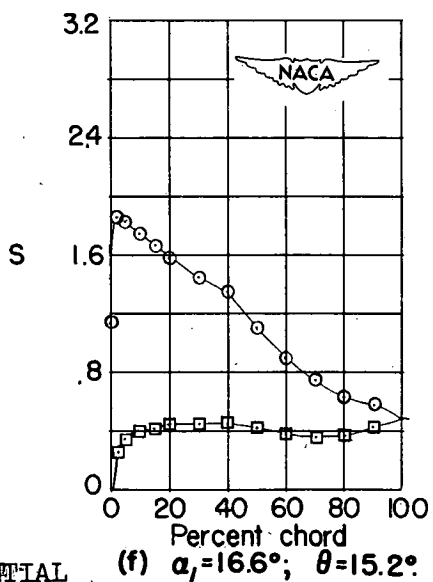
Figure 74.- Blade-surface pressure distributions and blade section characteristics for the cascade combination, \beta_1 = 70^\circ , \sigma = 1.00 , and blade section, NACA 65-(12)10.
