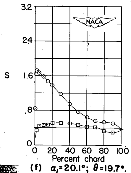
Figure 83.- Blade-surface pressure distributions and blade section characteristics for the cascade combination, \beta_1 = 70^\circ , \sigma = 1.50 , and blade section, NACA 65-(12)10.
