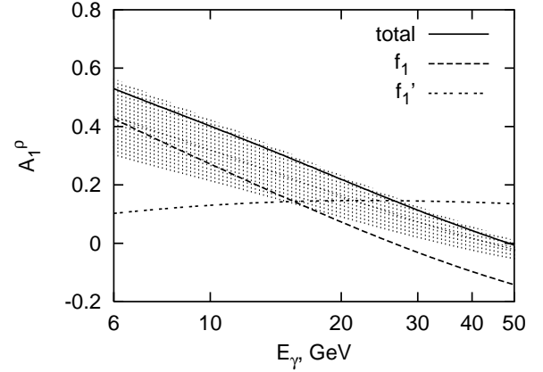
FIG. 7: The E_{\gamma^*} -dependence of the double-spin asymmetry A_1^p on the deuteron is shown. The notations are the same as in Fig. 6.
