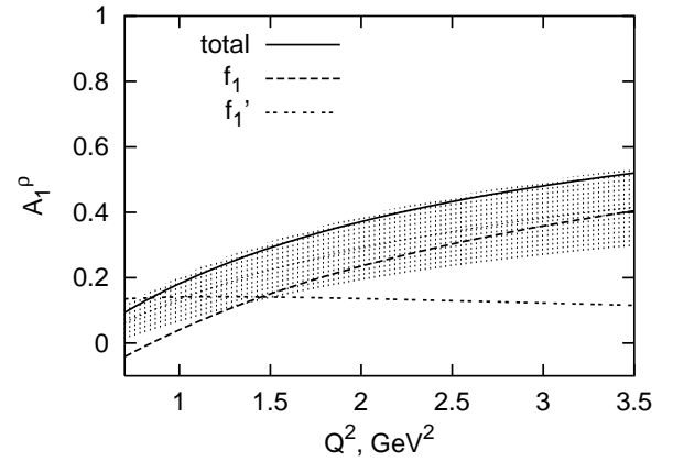
FIG. 9: The Q^2 -dependence of the double-spin asymmetry A_1^p on the deuteron is shown. The notations are the same as in Fig. 6.
