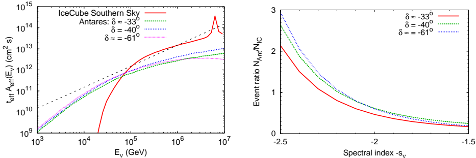
Figure 1: (left) Relative exposures of the ANTARES CLS [Adrián-Martínez et al., 2012] to a flavour-uniform neutrino flux from the characteristic declinations of the six blazars of Table 2, and the Southern-Sky-average of the IceCube HESE analysis [Aartsen et al., 2014a] (exposures from IceCube Collaboration [2013]). The black dashed line, included for reference purposes, is proportional to E_\nu . (right) Expected number of ANTARES events per detected IceCube event for power-law spectra (Eq. 1) as a function of the neutrino spectral index -s_\nu , calculated using the relative exposures.
