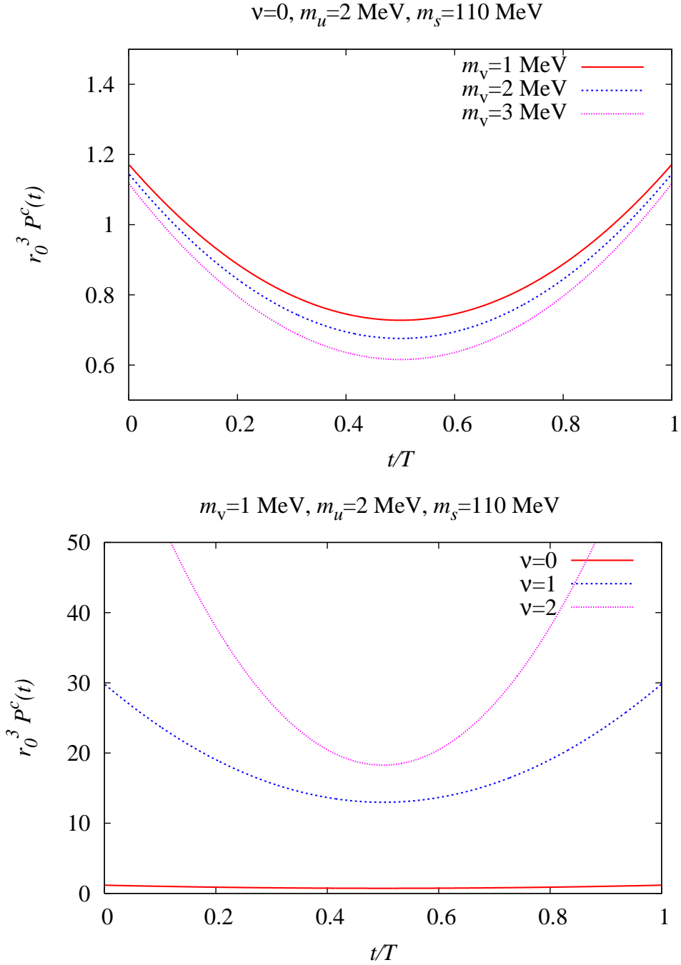
Figure 3: The pseudoscalar correlators with m_\nu = 1\text{-}3 \text{ MeV} , m_u = m_d = 2 \text{ MeV} and m_s = 110 \text{ MeV} in a sector of trivial topology, \nu = 0 (top) and in sectors of \nu = 0\text{-}2 for fixed m_\nu = 1 \text{ MeV} (bottom). We set L = T/2 = 2 \text{ fm} and the correlators are normalized by the Sommer scale r_0 = 0.49 \text{ fm} [48].
