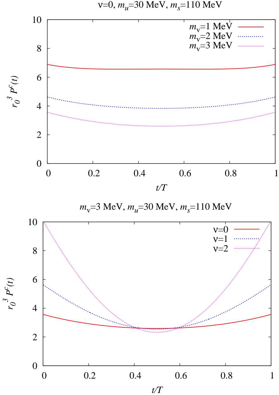
Figure 5: The pseudoscalar correlators with m_v = 1-3 \text{ MeV} , m_u = m_d = 30 \text{ MeV} and m_s = 110 \text{ MeV} in a sector of trivial topology, \nu = 0 (top) and in sectors of \nu = 0-2 for fixed m_v = 3 \text{ MeV} (bottom).
