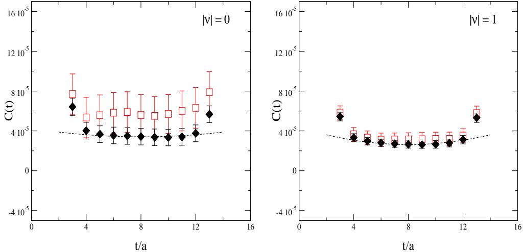
Figure 4: Left-left correlators in the \epsilon -regime for am = 0.005 , |\nu| = 0 (left) and |\nu| = 1 (right), computed with LMA (filled diamonds) and in the standard manner (open squares). The dashed lines represent fits to LMA data (see main text).
