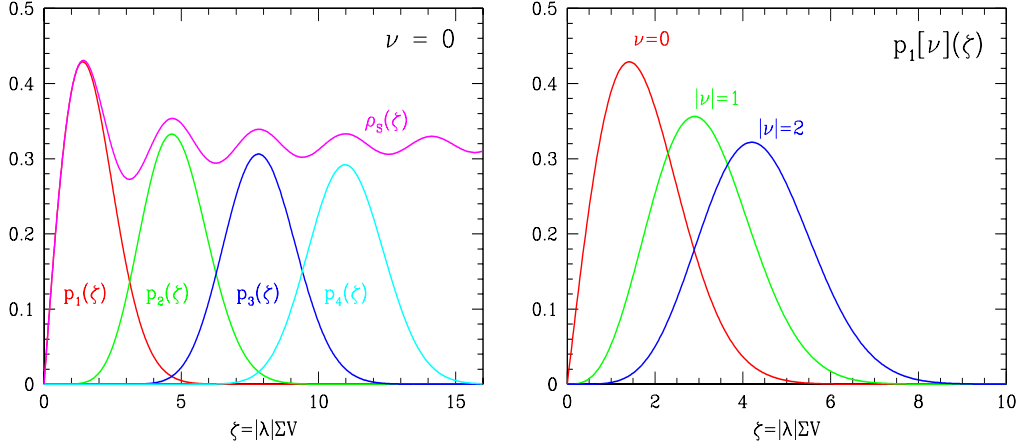
Figure 1: Probability density distributions of low-lying eigenvalues in quenched QCD. Left: distributions of the first four eigenvalues p_i(\zeta) ( i = 1, \dots, 4 ) and of the microscopic total density \rho_s(\zeta) for \nu = 0 . Right: distributions of the first eigenvalue for |\nu| = 0, 1, 2 .
