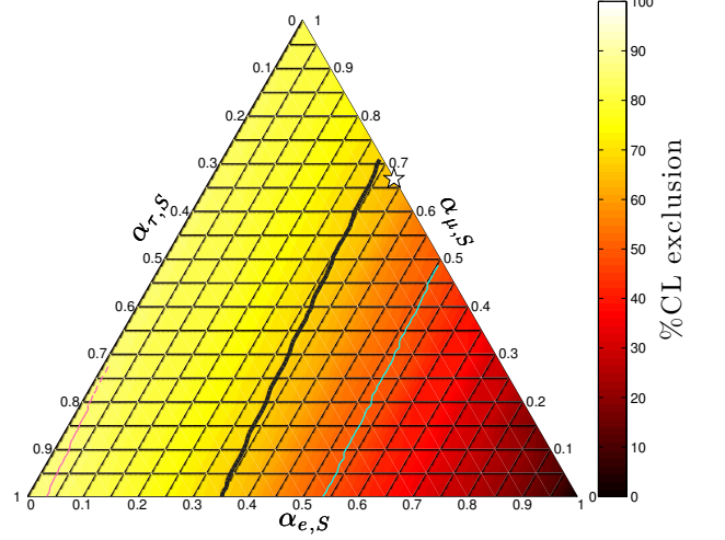
FIG. 2. Same as Fig. 1, but for \{\alpha_{i,S}\} at the source and assuming the signal neutrinos are astrophysical and oscillation probabilities are in the averaged regime, i.e., the parameter space is restricted to the blue sliver shown in Fig. 1. The best-fit is the darkest point, (1 : 0 : 0)_S . The white star corresponds to the (1 : 2 : 0)_S flavor combination. Standard flavor compositions lie within a narrow band along the right side of the triangle. Note that all combinations are allowed at 95% C.L. for the three spectra, and even at 68% C.L. for E_{\nu}^{-3} .
