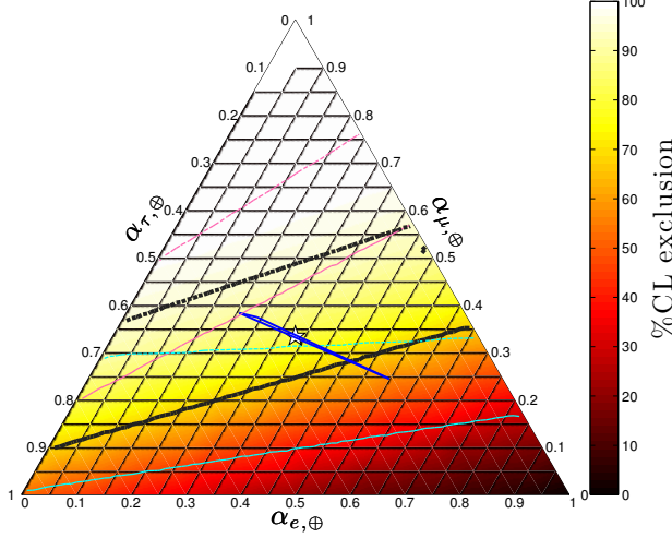
FIG. 1. Ternary plot of the exclusion C.L. for all possible flavor combinations ( \alpha_{e,\oplus} : \alpha_{\mu,\oplus} : \alpha_{\tau,\oplus} ) as seen at Earth, given the 7 tracks and 21 showers observed at IceCube. The lower right corner corresponds to 100% electron neutrinos, the upper corner is 100% muon neutrinos, and the lower left corner to 100% tau neutrinos. The central sliver outlined in blue corresponds to the possible flavor combinations for astrophysical neutrinos, after oscillations have been averaged during propagation. The best-fit is the darkest point, (1 : 0 : 0)_{\oplus} . The white star corresponds to (1 : 1 : 1)_{\oplus} , which is expected from a (1 : 2 : 0)_S combination at the source. The color scale indicates the exclusion C.L. given an E_{\nu}^{-2} spectrum of incoming neutrinos. Solid (dashed) lines show 68% C.L. (95% C.L.) contours, cyan for E_{\nu}^{-1} , thick black for E_{\nu}^{-2} and pink for E_{\nu}^{-3} spectra.
