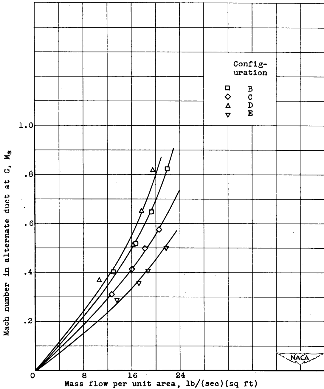
Figure 6. - Variation of alternate-duct Mach number with mass flow per unit air-flow area at compressor inlet. Main duct blocked; airspeed, 250 miles per hour; angle of attack, 0^\circ .
