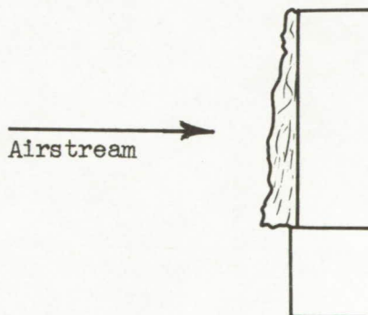
(b) Configuration E; round-wire screen; icing period, 11 minutes; initial mass flow per unit area, 24.5 pounds per second per square foot.
