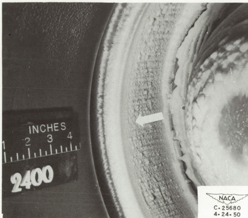
Figure 13. - Typical ice formations on duct-splitter ring of inertia-separation inlets. Round-wire screen; temperature, 10^{\circ} F; airspeed, 250 miles per hour; liquid-water content, 0.6 gram per cubic meter; icing period, 11 minutes; initial mass flow per unit area, 23.7 pounds per second per square foot.
