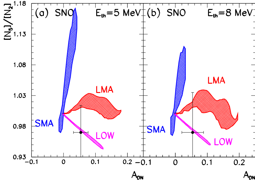
FIG. 13. The allowed values for the day–night asymmetry, A_{DN} and the ratio of rates in the N5 and N2 bins, N_5/N_2 , at SNO above 5 MeV (a) and 8 MeV (b) in the different allowed regions (at 99% CL) of the solar neutrino problem. We also show the expected statistical sensitivity after 3 years of operation (see text for details).
