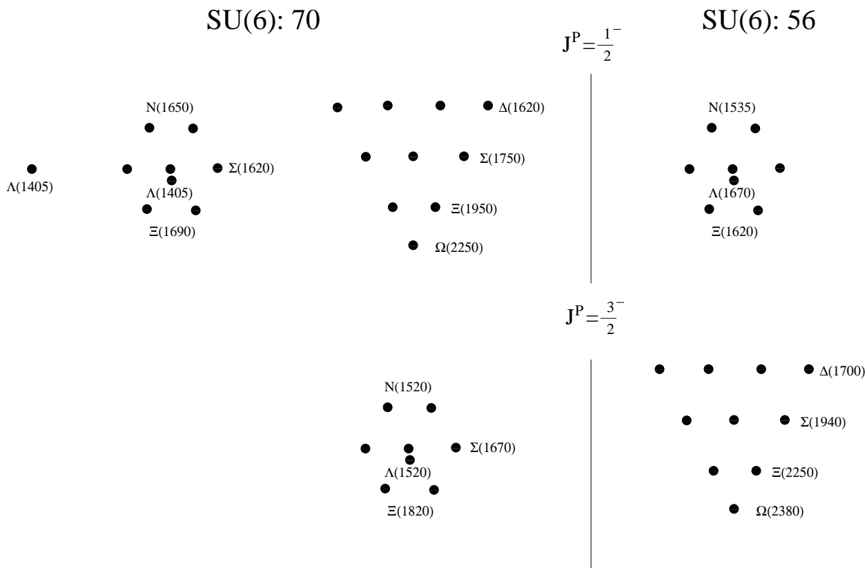
FIG. 1: Qualitative SU(6) classification derived from this work for the experimental low-lying \frac{1}{2}^- and \frac{3}{2}^- baryon resonances. This classification is made attending to the relation of each resonance with the different SU(6)/SU(3) multiplets that appear in the spin and/or flavor symmetric scenario described in Sect. III. Most of the odd parity three and four star resonances of the PDG are included. Few two star ( \Sigma(1620) , \Xi(2250) , and \Omega(2380) ) and one star ( \Xi(1620) ) resonances complete the SU(6) multiplets. The only exception is the missing \Sigma state in the \frac{1}{2}^- octet of the 56. The classification predicts the experimentally not yet known spin-parity of five resonances: \Xi(1620) , \Xi(1690) , \Xi(1950) , \Xi(2250) , \Omega(2250) , and \Omega(2380) . Most of the resonances have large SU(6) and SU(3) mixing.
