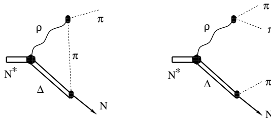
FIG. 3: Resonance ( N^* ) decay to \pi N (left) or \pi\pi\pi N (right) through its s -wave (hexagon) coupling to \Delta\rho and the p -wave coupling (ovals) of these latter hadrons to two pions and to a \pi N pair.
