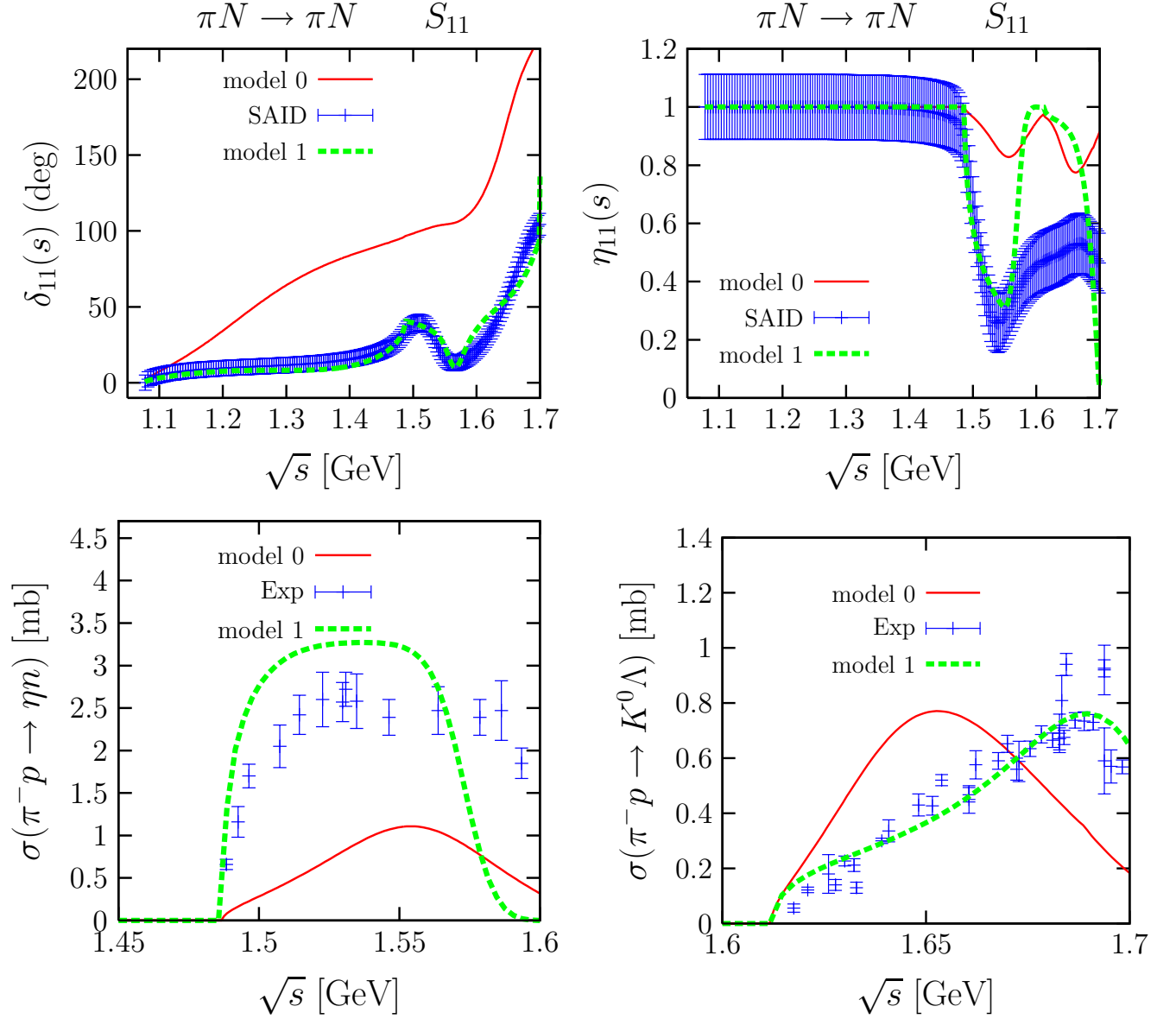
FIG. 4: Top panels: S_{11} -elastic \pi N phase shifts (left) and inelasticities (right) as a function of the C.M. energy \sqrt{s} . Data are from Ref. [53], and to better appreciate the discrepancies, we have assumed in both cases a 5% systematic error and a statistical uncertainty of 5^\circ and 0.1 for \delta's and \eta's , respectively (errors have been added in quadrature). Bottom panels: \pi^- p \rightarrow \eta n and \pi^- p \rightarrow K^0 \Lambda total cross sections as a function of \sqrt{s} . Data are from Ref. [47]. Solid lines (model 0) stand for the predictions obtained within the scheme presented here, where no parameters have been adjusted to data. Dashed lines (model 1) show results from a modified model, where in Eq. (14), the subtraction constants \bar{J}_0(\mu = \sqrt{m_\pi^2 + M_N^2}; M_i, m_i) are multiplied by the factors -0.039, 0.007, 2.228, -0.539, 0.443, 0.757, 2.855, 0.710, 1.460, 2.677, 0.333 , for the \pi N, \eta N, K\Lambda, K\Sigma, \rho N, \omega N, \phi N, \rho\Delta, K^*\Lambda, K^*\Sigma, K^*\Sigma^* channels, respectively.
