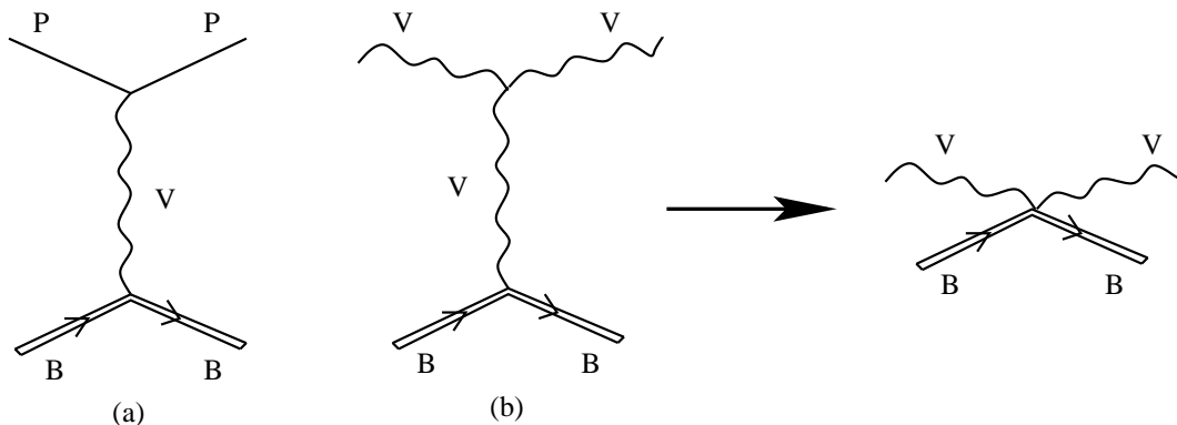
FIG. 2: Diagrams contributing to the pseudoscalar-baryon (a) or vector-baryon (b) interaction via the exchange of a vector meson leading to the effective vector-baryon contact interaction.
