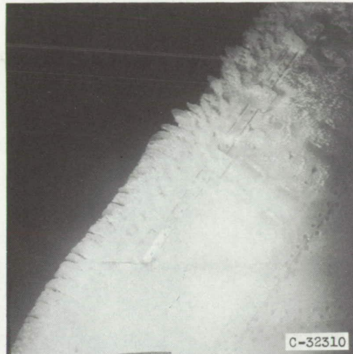
Lower surface. Icing time, 11 minutes; section drag coefficient, 0.0360.
