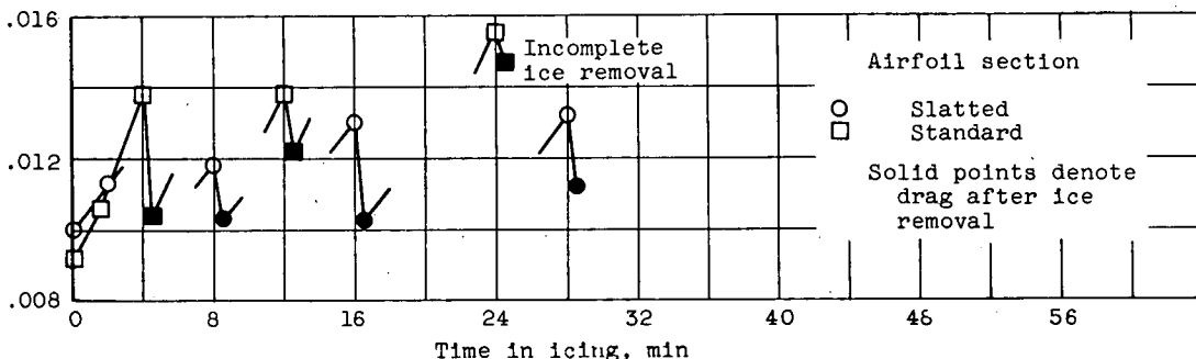
(c) Angle of attack, 2°; liquid-water content, 0.80 gram per cubic meter; icing period, 220 seconds; heat-on period, 20 seconds.
