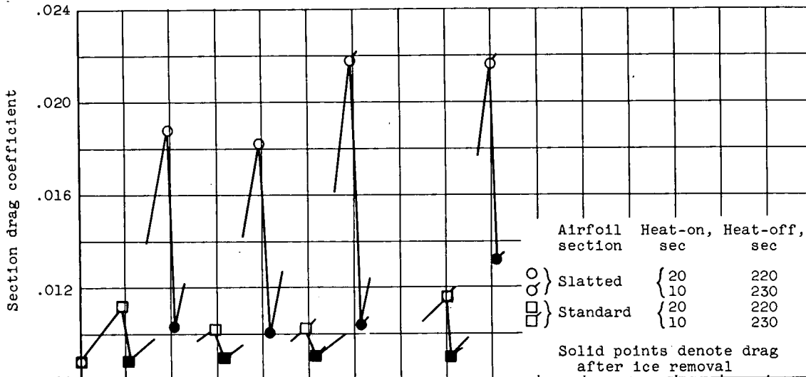
(b) Angle of attack, 4°; liquid-water content, 0.80 gram per cubic meter.
