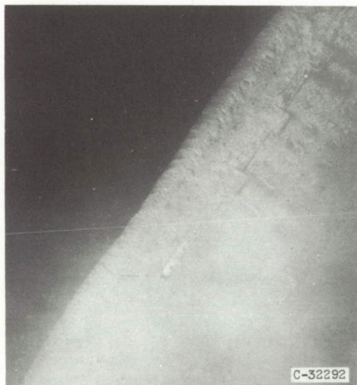
Lower surface. Icing time, 10 minutes; section drag coefficient, 0.0252.
