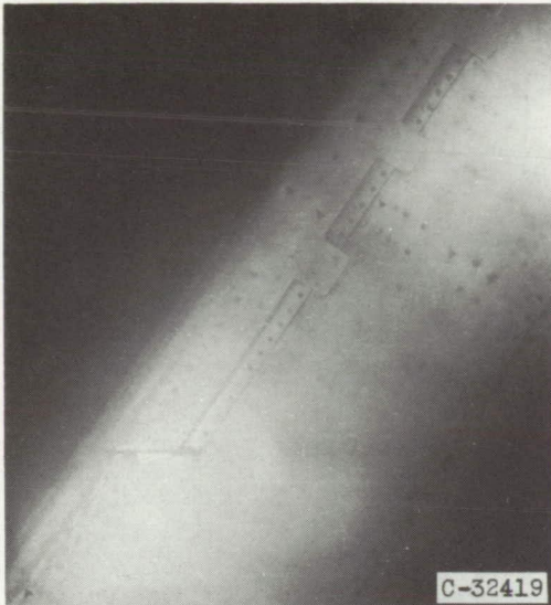
Lower surface. Icing time, 12 minutes; section drag coefficient, 0.0138; before ice removal; standard airfoil.
