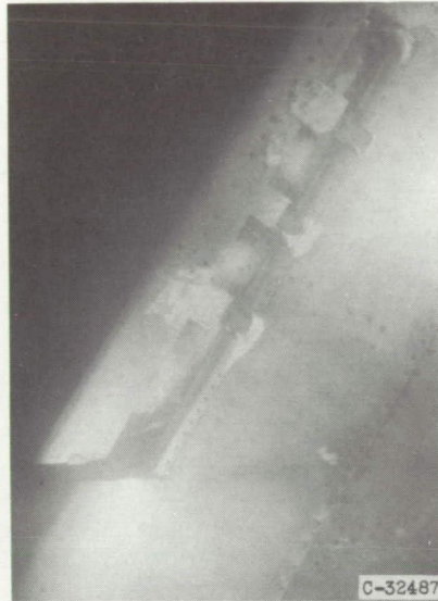
Lower surface. Icing time, 33 minutes; after ice removal.
