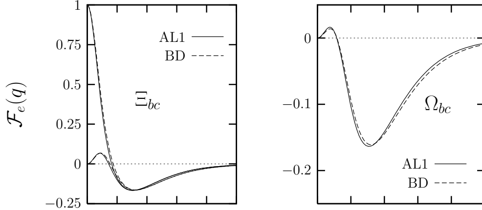
FIG. 4: Charge form factor of the \Xi_{bc} and \Omega_{bc} baryons evaluated with the AL1 (solid line) and BD (dashed line) potentials. For \Xi_{bc} baryons we show the two possible charge states. Similar results are obtained for \Xi_{bc}^* , \Xi_{bc} and \Omega_{bc}^* , \Omega_{bc} .
