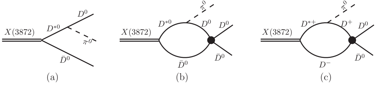
FIG. 2. Feynman diagrams for the decay X(3872) \rightarrow D^0 \bar{D}^0 \pi^0 . The charge conjugate channel is not shown but included in the calculations.
