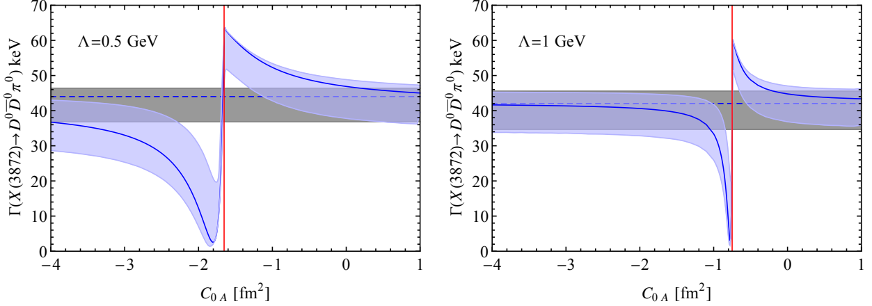
FIG. 3. Dependence of the X(3872) \rightarrow D^0 \bar{D}^0 \pi^0 partial decay width on the low-energy constant C_{0A} . The UV cutoff is set to \Lambda = 0.5 GeV (1 GeV) in the left (right) panel. The blue error bands contain D\bar{D} FSI effects, while the grey bands stand for the tree level predictions of Eq. (19). The solid (full calculation) and dashed (tree level) lines stand for the results obtained with the central values of the parameters. The vertical lines denote the values of C_{0A} for which a D\bar{D} bound state is generated at the D^0 \bar{D}^0 threshold.
