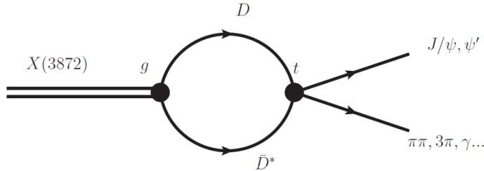
FIG. 1. Mechanism for the decays of the X(3872) into J/\psi\pi\pi , J/\psi3\pi , J/\psi\gamma , \psi'\gamma ... assuming the X(3872) to be a D\bar{D}^* molecule. The charge conjugated channel is not plotted.
