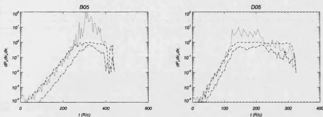
Figure 3.48: Pressure and axial and radial velocity perturbation evolution for several modes simulations. Left panel: model B05. Right panel: model D05.
