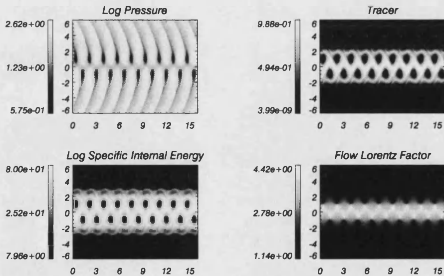
Figure 2.45: Same as Fig. (2.26) for models B05 (upper) and D05 (lower) perturbed with first body antisymmetric mode, at the end of simulations.
