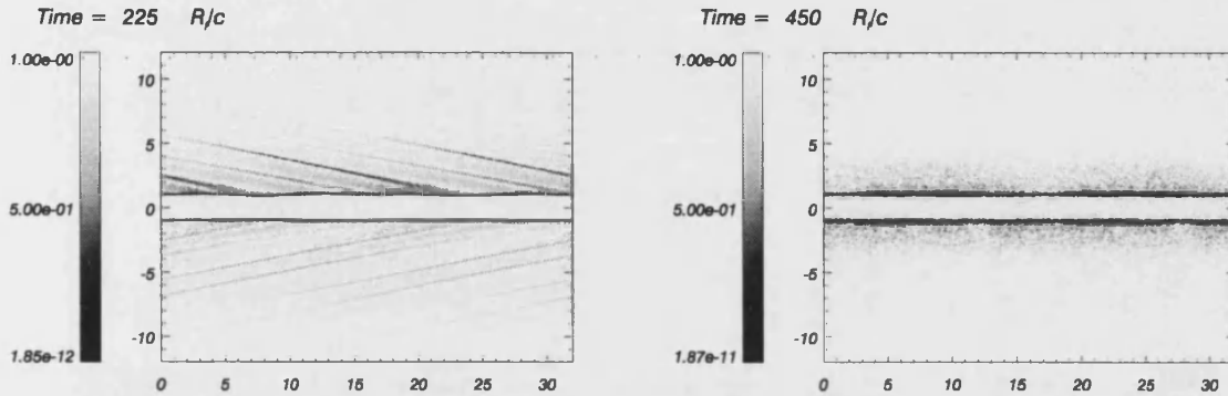
Figure 3.29: Schlieren plots showing waves in the linear regime in models B05 (left) and B20 (right). Long wavelength structures in B05 are apparent, contrary to small structures in B20 . These plots represent a negative exponential of the density gradient times an arbitrary factor chosen for the sake of clarity ( \exp(-k|\nabla\rho|) , with k = 30 ). Thus 1.0 means no density gradient and the lowest value stands for maximum density gradient.
