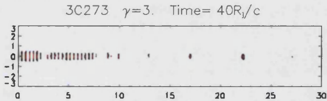
Figure 4.10: Surface plot of Lorentz factor \gamma = 3.0 at t = 40 R_j/c .
