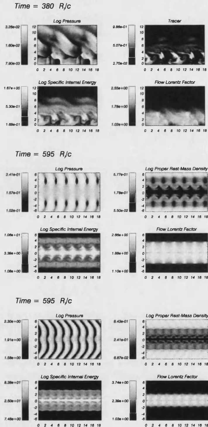
Figure 2.27: Same as Fig. (2.26) for models B05 (upper; only top half of the model shown), C05 (middle) and D05 (lower).
