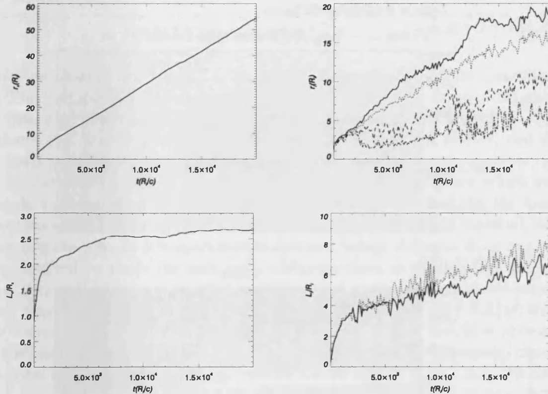
Figure 4.15: Top left panel stands for the mean cavity radius, and top right panel for the mean jet radius (different lines stand for the different criteria used to fix the jet head position: solid line is for tracer f = 0.01 , dotted line for f = 0.1 , dashed line for f = 0.5 and dash-dotted line for f = 0.9 ). Bottom panels stand for cavity shape (left) and jet shape (right). See text.
