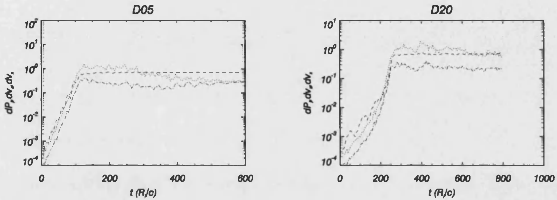
Figure 2.43: Same as Fig 2.42 for models D05 (left panel) and D20 (right panel).
