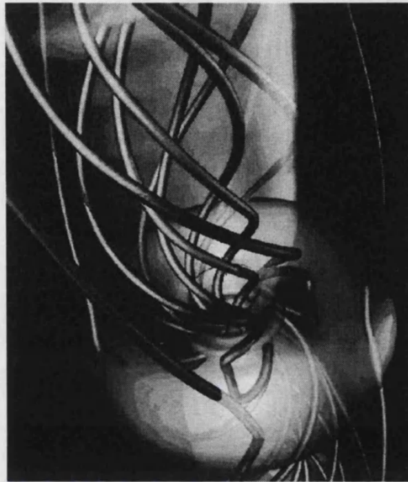
Figure 1.6: Caption from a simulation of jet formation in the surroundings of a SMBH; lines stand for magnetic field (Meier et al. 2001).
