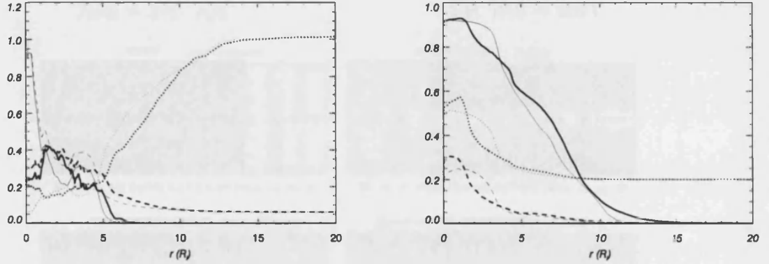
Figure 2.38: Longitudinal averaged profiles of relevant physical quantities for models C16 (thin lines) and C128 (thick lines) in the last snapshot of simulation C128 ( t = 375R_j/c ). Left panel: tracer (full line), rest mass density (dotted line) and internal energy divided by 10 (dashed line). Mixing produces a denser and colder jet in model C128. Right panel: longitudinal velocity (full line), Lorentz factor normalized to its initial value (dotted line) and longitudinal momentum normalized to its initial value (dashed line).
