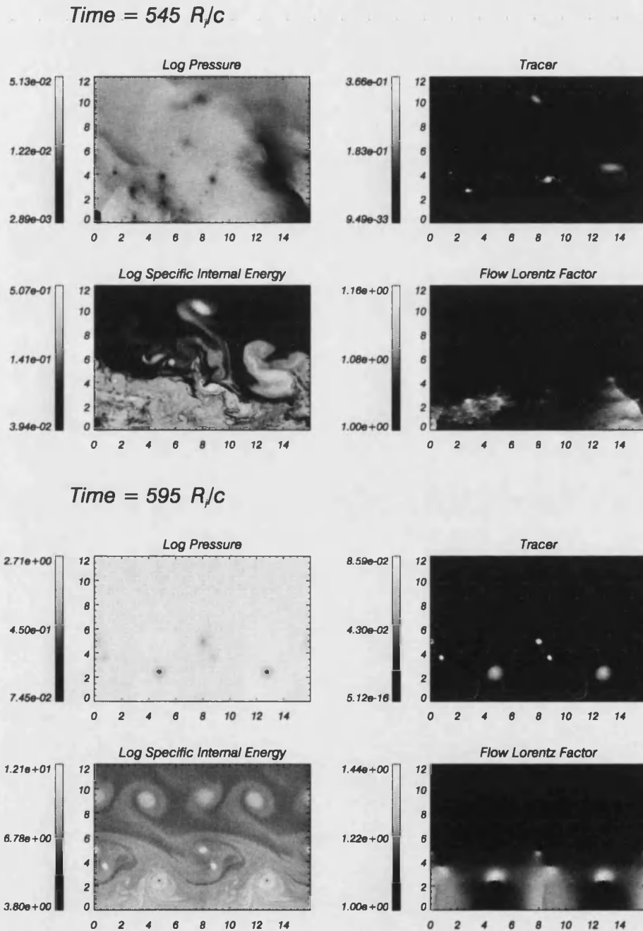
Figure 3.51: Snapshot at the last frame of the simulation of logarithmic maps of pressure, jet mass fraction and specific internal energy and non-logarithmic Lorentz factor for cylindrical models B05 (upper) and D05 (lower).
