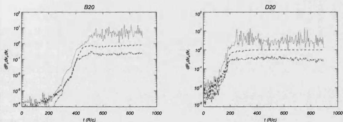
Figure 3.49: Same as Fig. 3.48. Left panel: model B20. Right panel: model D20.
