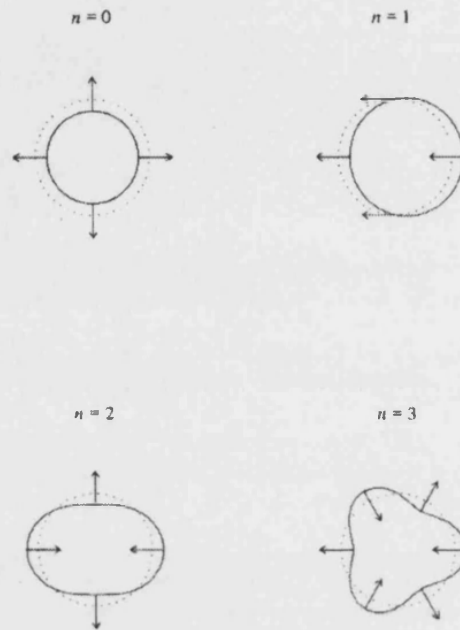
Figure 2.7: Deformations of jets by Kelvin-Helmholtz instability modes (from Birkinshaw 1991b).
