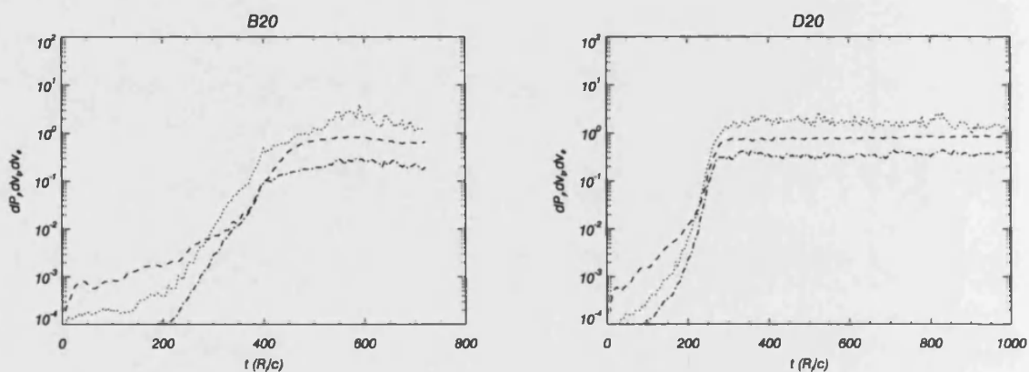
Figure 3.27: Same as Fig. 3.23 for models B20 and D20 .
