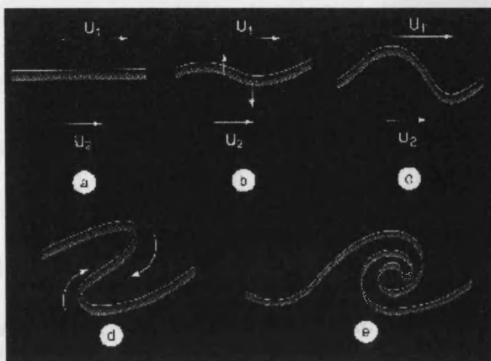
Figure 1.11: Development of Kelvin-Helmholtz instability.
