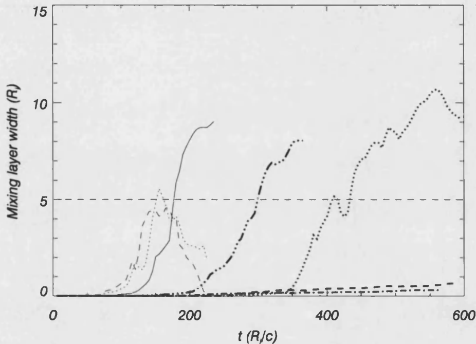
Figure 2.22: Same as Fig. 2.15, for models F, G, H, I, J, K and L. Different types of lines are used for models with different internal energies: Continuous line: model F; dotted line: model G; dashed line: model H; thick dotted line: model I; thick dashed line: model J; thick dashed-dotted line: model K; thick dash-dot-dot line: model L. A value of 5 R_j for the width of the mixing layer (horizontal dashed line) serves to classify the evolution of the different models.
