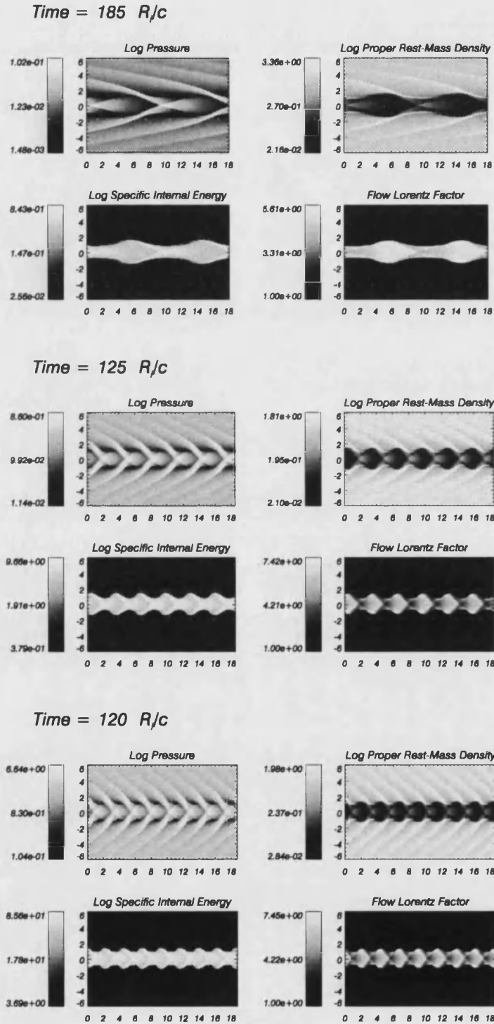
Figure 2.12: Same as Fig. (2.11) for models B05 (upper), C05 (middle) and D05 (lower).
