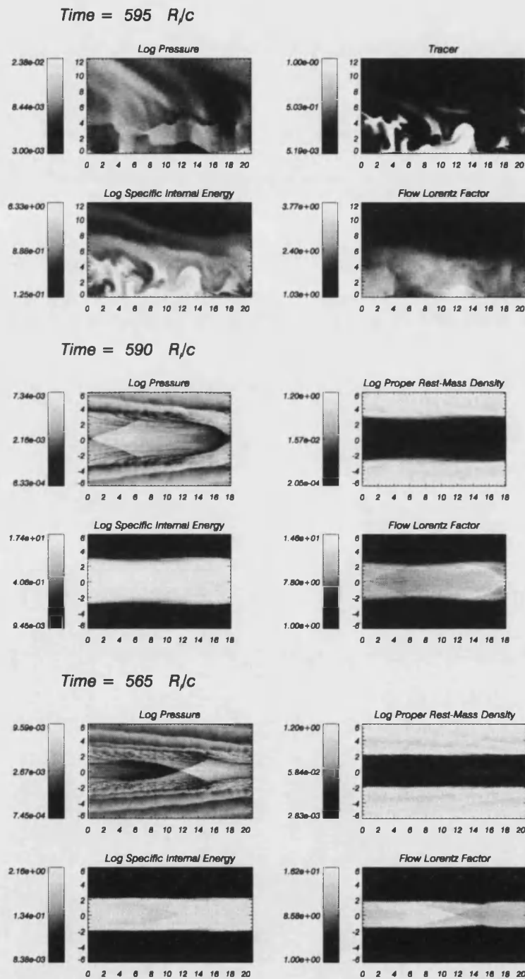
Figure 2.31: Same as Fig. (2.26) for models I (upper), and J (middle) and K (lower); only top half of the model shown for I).
