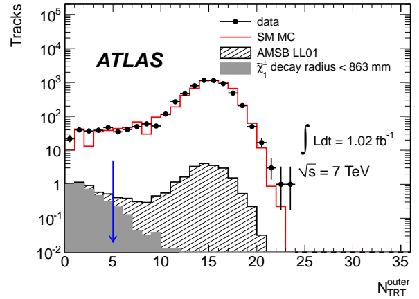
Fig. 1 The N_{\text{TRT}}^{\text{outer}} distribution for data and signal events (LL01, \tau_{\chi_1^\pm} = 1 ns) with the high- p_T isolated track selection. The selection boundary is indicated by the arrow. The expectation from SM MC events, normalized to the number of observed events, is also shown. When charginos decay before reaching the TRT outer module, N_{\text{TRT}}^{\text{outer}} is expected to have a value near zero; conversely, SM charged particles traversing the TRT typically have N_{\text{TRT}}^{\text{outer}} \simeq 15 .
