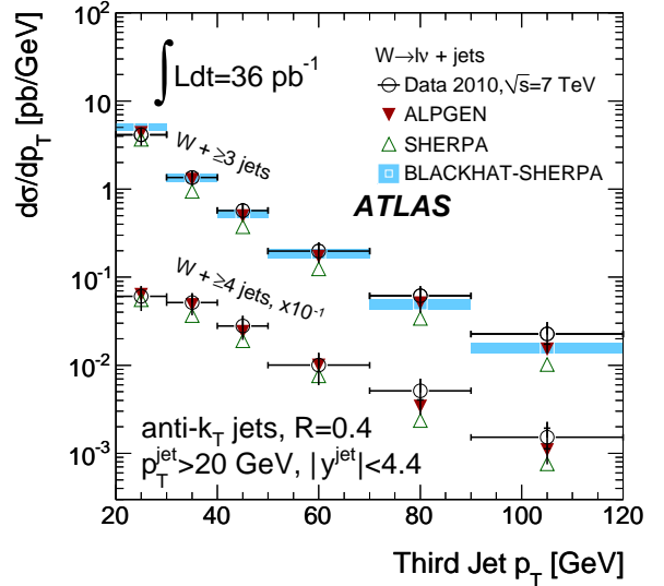
FIG. 37. W +jets cross section as a function of the p_T of the third jet in the event. The p_T of the third jet is shown separately for events with \geq 3 jet and \geq 4 jet. The \geq 4 jet distribution has been scaled down by a factor of 10. Shown are predictions from ALPGEN, SHERPA, and BLACKHAT-SHERPA.
