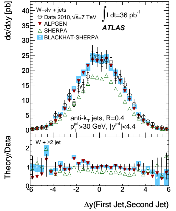
FIG. 31. W +jets cross section as a function of y (first jet) – y (second jet) for events with \geq 2 jets. Shown are predictions from ALPGEN, SHERPA, and BLACKHAT-SHERPA, and the ratio of theoretical predictions to data.
