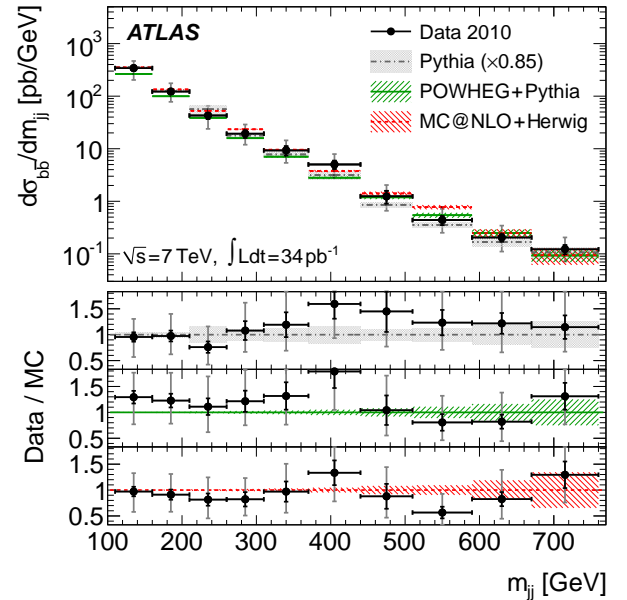
Fig. 6. The b\bar{b} -dijet cross-section as a function of dijet invariant mass for b -jets with p_T > 40 GeV and |y| < 2.1 . The data are compared to the MC predictions of Pythia, POWHEG and MC@NLO. The leading-order Pythia prediction is scaled to the measured integrated cross-section. The shaded regions around the MC predictions reflect the statistical uncertainty only.
