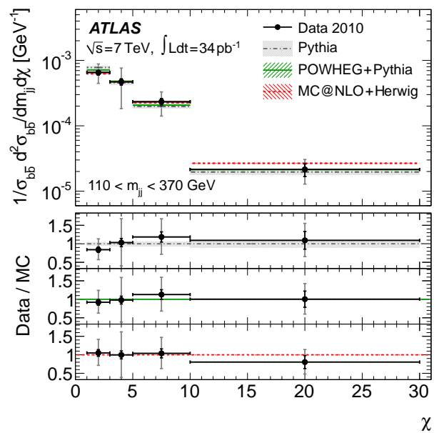
(a) 110 < m_{jj} < 370 GeV
