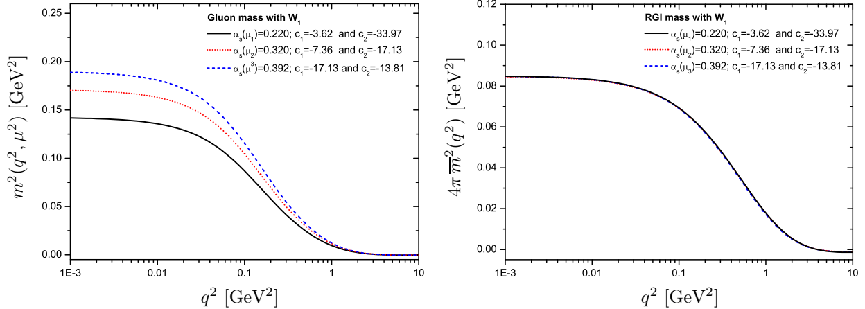
FIG. 8: (color online) The gluon dynamical mass m^2(q^2, \mu^2) (left panel) and the corresponding RGI mass 4\pi \overline{m}^2(q^2) (right panel) obtained using the model of Eq. (6.6) for the three values of \mu_i .
