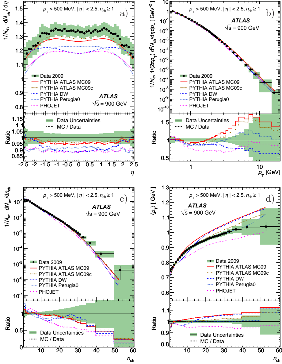
Figure 3: Charged-particle multiplicities for events with n_{\text{ch}} \geq 1 within the kinematic range p_{\text{T}} > 500 MeV and |\eta| < 2.5 . The panels show the charged-particle multiplicity as a function of pseudorapidity (a) and of the transverse momentum (b), the charged-particle multiplicity (c), and the average transverse momentum as a function of the number of charged particles in the event (d). The dots represent the data and the curves the predictions from different MC models. The vertical bars represent the statistical uncertainties, while the shaded areas show statistical and systematic uncertainties added in quadrature. The values of the ratio histograms refer to the bin centroids.
