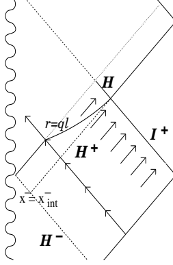
FIG.2. Penrose diagram corresponding to the process of particle capture by an extremal charged black hole followed by Hawking radiation. The end-state geometry is, due to backreaction effects, an extremal black hole. The location of the event horizon H^+ is at x^- = x^-_{int} .
