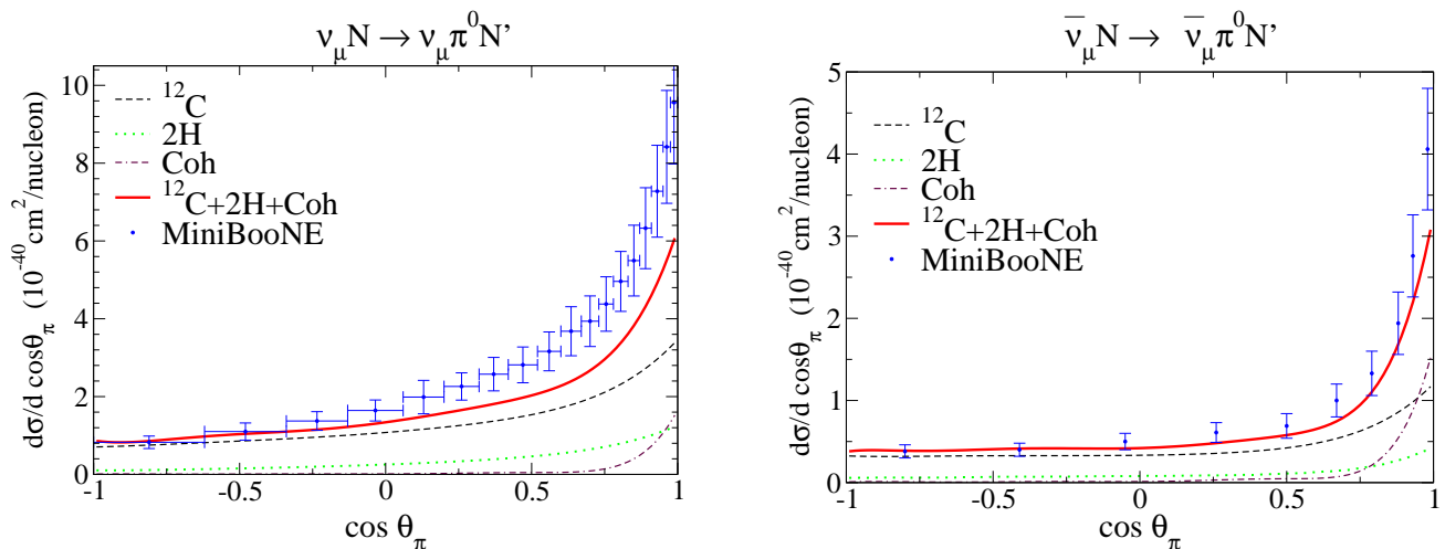
FIG. 10. Flux-folded differential \frac{d\sigma}{d\cos\theta_\pi} cross section per nucleon for NC\ 1\pi^0 production by \nu_\mu (left panel) and \bar{\nu}_\mu (right panel) in mineral oil. Captions as in Fig. 9. Data from Ref. [2].
