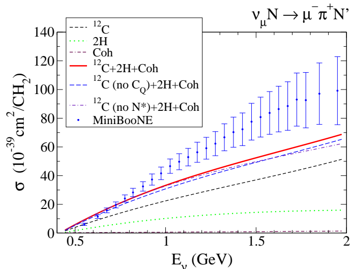
FIG. 4. 1\pi^+ total production cross section for \nu_\mu CC interaction in mineral oil. Short-dashed line: ^{12}\text{C} contribution. Dotted line: \text{H}_2 contribution. Double-dashed dotted line: Coherent contribution (see main text). Solid line: Total contribution. Long-dashed line: Same as solid line but without the C_Q contribution of Eq. (11). Dashed-dotted line: Same as solid line but without the contribution from the D_{13} resonance contribution. Data taken from Ref. [3].
