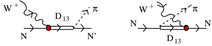
FIG. 3. D_{13}(1520) contributions to W^+N \rightarrow N'\pi . We have direct ( DP ) and crossed ( CDP ) D_{13}(1520) -pole contributions.
