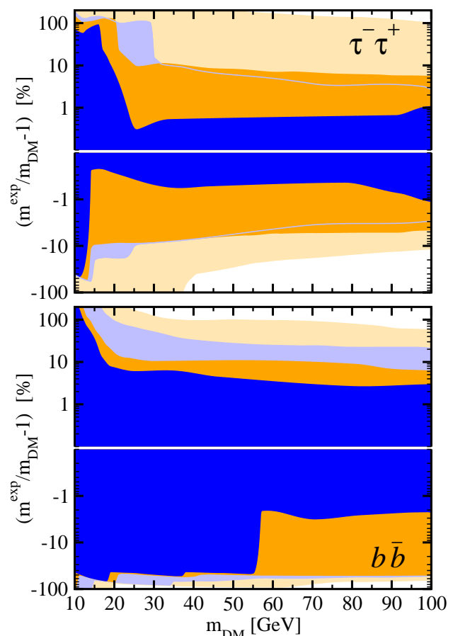
Figure 1: Relative error in the DM mass after 10 years at DeepCore at 90% CL, with (light colors) and without (dark colors) systematic errors. Top panel: Annihilations into \tau^-\tau^+ with \sigma_{SD}^p = 10^{-3} pb (blue), 10^{-4} pb (orange). Bottom panel: Annihilations into b\bar{b} with \sigma_{SD}^p = 10^{-2} pb (blue), 4 \times 10^{-3} pb (orange).
