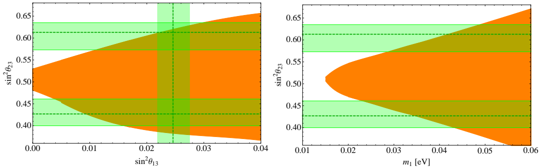
Figure 2: Correlations between the atmospheric angle, and the reactor angle (left panel) and the lightest neutrino mass (right panel). Straight bands are the currently allowed 1\sigma bands of the oscillation angles, taken from Ref. [13].
