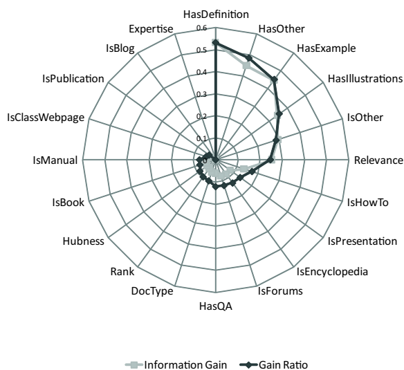
Fig. 3: Information gain for user-features
