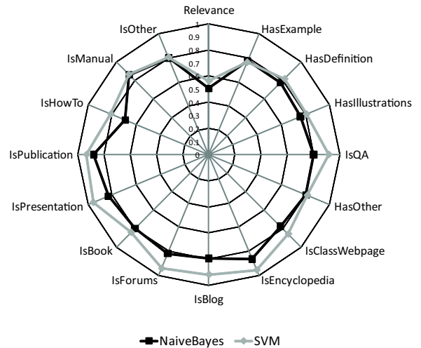
Fig. 2: Classification results for user-features
