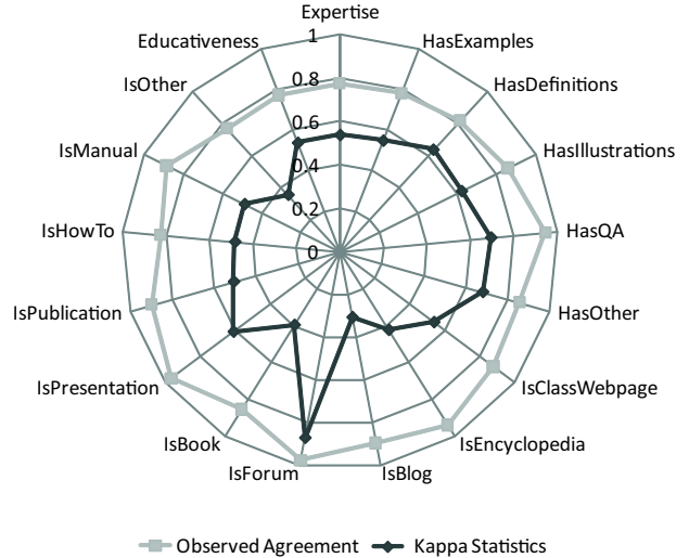
Fig. 1: Kappa statistic and inter-annotator agreement
