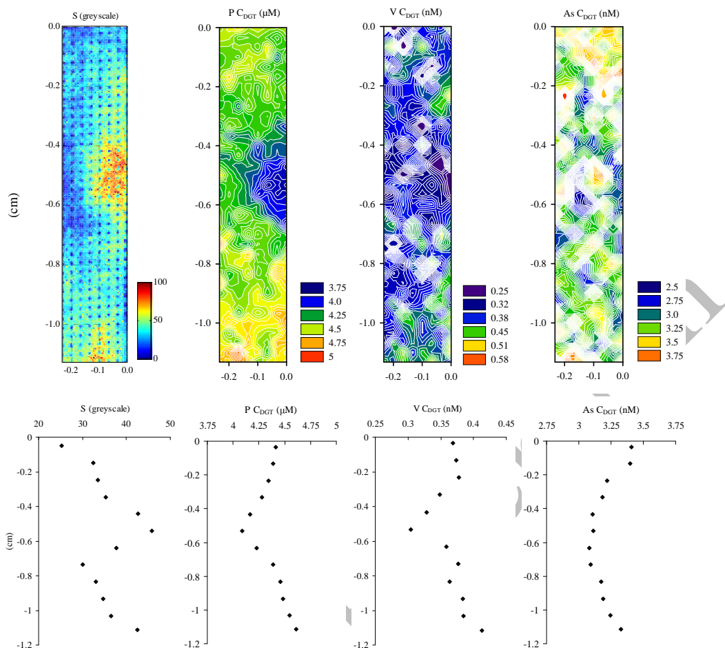
Figure 2. Analyte profiles at a microniche. 2-D images show greyscale density for sulphide and DGT resolved concentrations ( C_{DGT} ) for P, V and As. The ablation grid (eight columns, 35 rows) can be seen on the sulphide scan with each point representing a data point for the 2D C_{DGT} figures. 1-D plots show concentration-depth profiles obtained by averaging the data into one-mm deep vertical slices (24 ablation spots per point, except the lowest point where the bottom two rows of ablation spots are averaged). Averaged greyscales values are affected, due to the ablation spots having low values. The elevated sulphide at the very bottom of the analysed area is possibly associated with a general elevation in sulphide at that depth, as such a feature was present across the entire width (18 mm) of the DGT probe for that depth coordinate (this work, unpublished data). Distances are in cm and are relative to the top right hand corner of the area.
