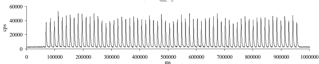
Figure 1. Time series of counts per second (cps) recorded by the mass spectrometer detector for a 64 spot ablation grid with 200 \mu\text{m} spacing of a standard gel exposed to 1.4 \text{nmol cm}^{-2} of P and 0.14 \text{nmol cm}^{-2} of V and As. Fe is used as the internal standard. Values for the residual standard deviation (RSD) are for the resolved peak areas before internal standardisation.
