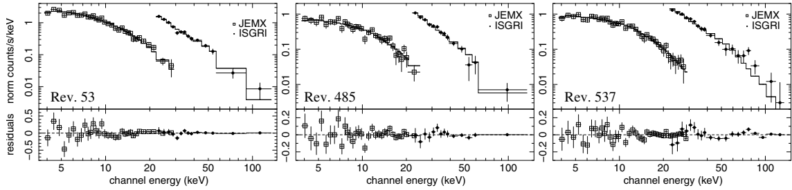
Fig. 6. Fit to the joint INTEGRAL /JEM-X plus INTEGRAL /ISGRI spectra from revolutions 53, 485, and 537. Residuals are in units of \text{count s}^{-1} \text{keV}^{-1} .
