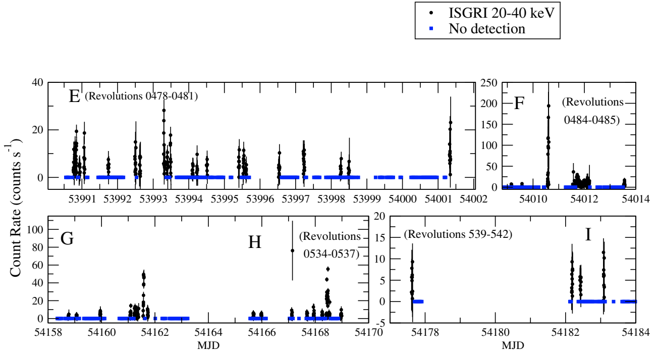
Fig. 2. Light curve of XTE J1739-302 data from INTEGRAL Key Programme 1 (KP1, September–November 2006 and February–March 2007). To reveal the number and structure of outbursts, a binning time of 200 s has been used.
