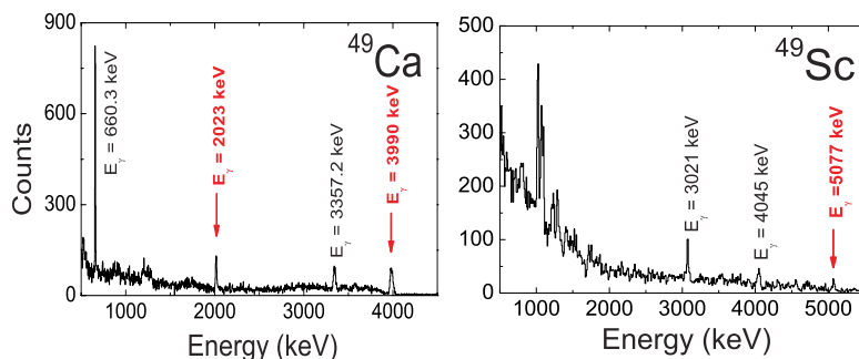
Fig. 2. Gamma spectra of ^{49}\text{Ca} (left) and ^{49}\text{Sc} (right). The arrows indicate the transitions which have been observed in reaction involving light ions only [6].
