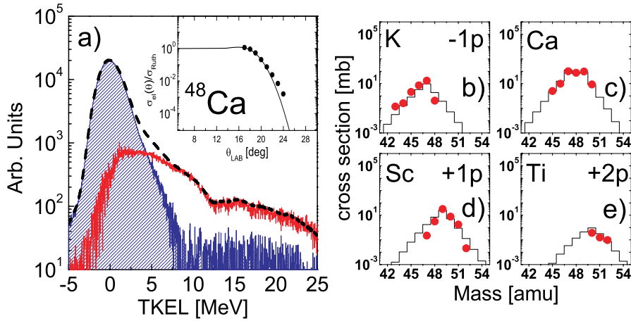
Fig. 1. Panel (a): the TKEL distribution of ^{48}\text{Ca} (angle-integrated) measured in PRISMA without coincidence with \gamma -rays (dashed line) and requiring a \gamma -coincidence in the Ge array (solid line). The difference spectrum (shaded area) gives the pure elastic scattering contribution. The points in the inset give the ratio of the elastic peak to the Rutherford cross-section over the angular acceptance of PRISMA, compared to the calculation by the GRAZING code [2]. Panels (b)–(e): experimental total cross-sections for some of the most intense transfer channels (symbols), compared to predictions by GRAZING (histograms).
