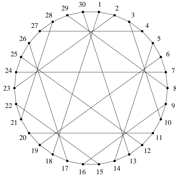
Figure 1: Tutte's (3, 8) cage
