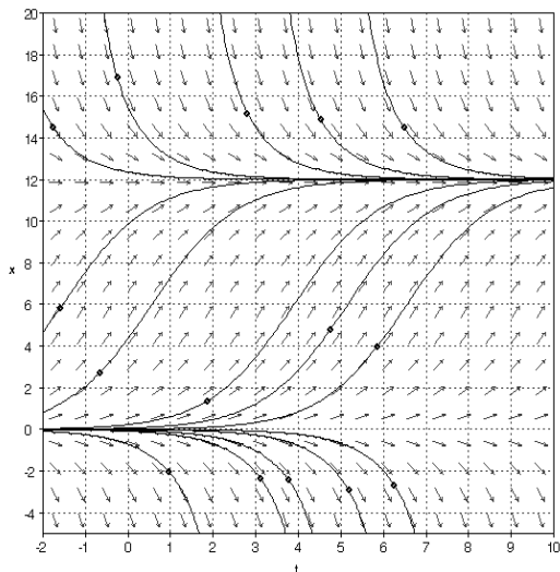
Figure 1: Slope field for a logistic model
