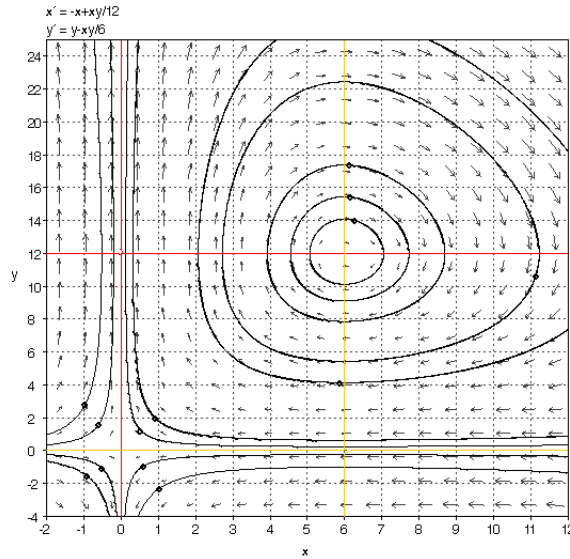
Figure 4: Some orbits in the predator prey phase plane
