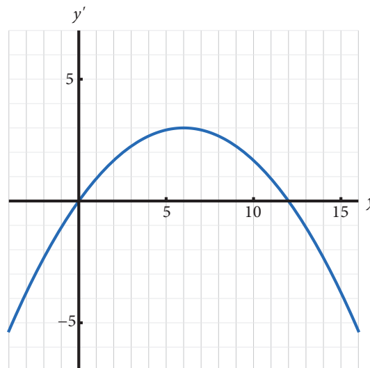
Figure 2: Phase plane for logistic model
