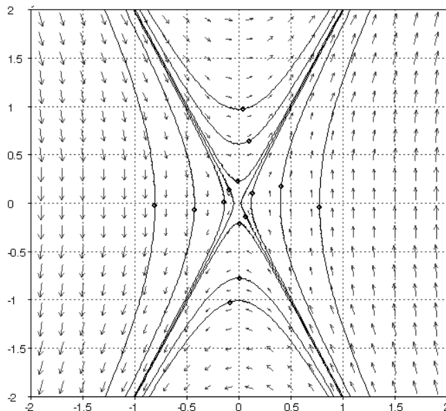
Figure 5: A big X made of eigenlines
