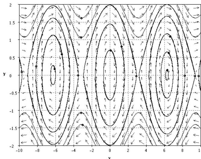
Figure 3: Frictionless Pendulum: x' = y , y' = -\sin x
