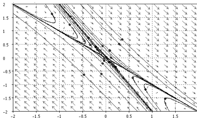
Figure 6: Two clear eigenlines again
