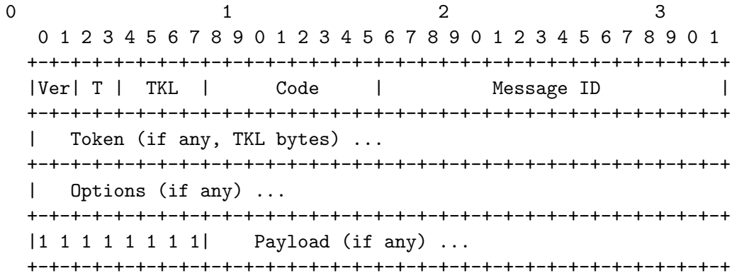
Figure 4.1: CoAP Message Format [1]
