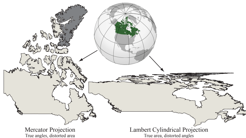
Figure 5: Two map projections of the outline of Canada, with Ellesmere Island shaded. The island’s shape is accurately depicted in the conformal Mercator projection, but its area relative to the rest of Canada is not: it comprises roughly 2% of Canada’s total land area but more than 13% of area on the Mercator map. The Lambert map depicts its relative area accurately, but distorts its shape. These distortions are especially pronounced due to the island’s proximity to the North Pole.
