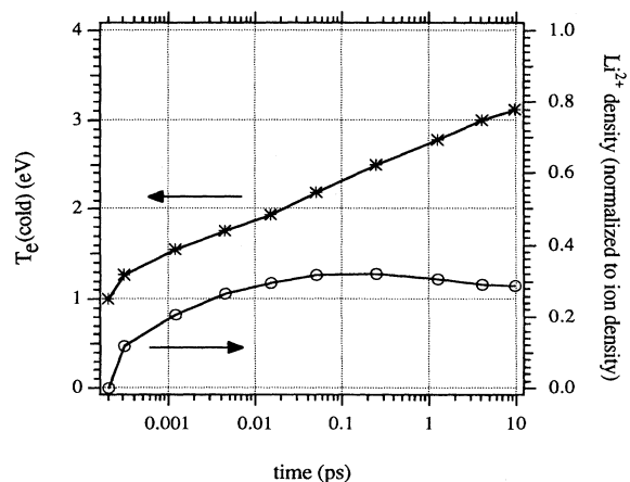
FIG. 4. T_e(\text{cold}) and fractional population of the recombined, H-like species, as functions of time. Conditions are the same as in Fig. 3(b).
