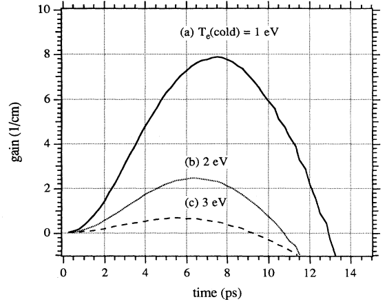
FIG. 2. Gain as a function of time for various fixed T_e(\text{cold}) , n_{\text{ion}} = 3.0 \times 10^{18} \text{ cm}^{-3} , n_e(\text{OFI}) = 6.0 \times 10^{18} \text{ cm}^{-3} , T_e(\text{OFI}) = 1 \text{ keV} , and n_e(\text{cold}) = 3.0 \times 10^{18} \text{ cm}^{-3} . The curves represent (a) T_e(\text{cold}) = 1 eV; (b) T_e(\text{cold}) = 2 eV; (c) T_e(\text{cold}) = 3 eV.
