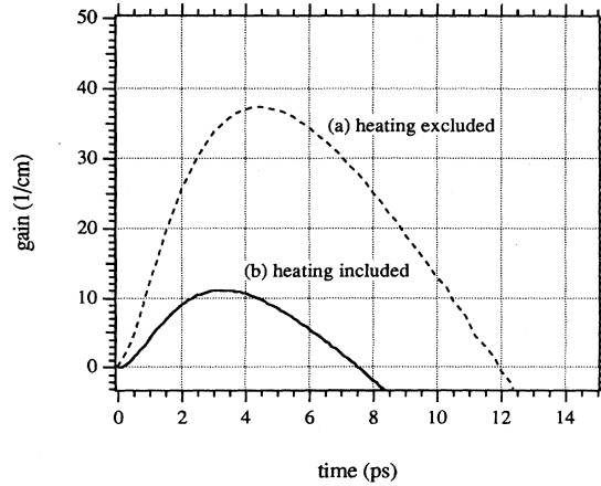
FIG. 3. Gain as a function of time with n_{\text{ion}} = 1 \times 10^{19} \text{ cm}^{-3} , n_e(\text{cold}) = 1 \times 10^{19} \text{ cm}^{-3} , T_e(\text{cold}) = 1 \text{ eV} , n_e(\text{OFI}) = 2 \times 10^{19} \text{ cm}^{-3} , and T_e(\text{OFI}) = 1 \text{ keV} for (a) no electron heating and (b) recombination and collisional electron heating included. Equilibration between the cold- and hot-electron distributions is ignored.
