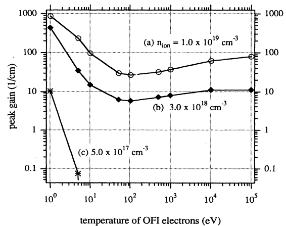
FIG. 1. Peak gain on the Ly- \alpha transition in \text{Li}^{2+} as a function of the OFI electron temperature. The cold-electron temperature [ T_e(\text{cold}) ] is held constant at 1 eV and \frac{1}{2} n_e(\text{OFI}) = n_e(\text{cold}) = n_{\text{ion}} . (a) n_{\text{ion}} = 1.0 \times 10^{19} \text{ cm}^{-3} ; (b) n_{\text{ion}} = 3.0 \times 10^{18} \text{ cm}^{-3} ; (c) n_{\text{ion}} = 5.0 \times 10^{17} \text{ cm}^{-3} .
