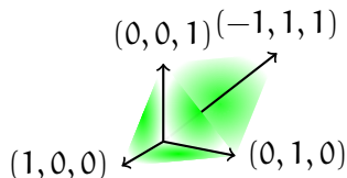
FIGURE 4. The fan of local \mathbb{P}^1
