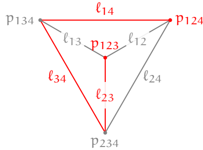
FIGURE 12. The torus-invariant subvarieties of \mathbb{P}^3 . The red subvarieties comprise the blowup locus for Class B, blown up in the following order: p_{123}, p_{124}, \ell_{23}, \ell_{34}, \ell_{14} .
