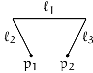
FIGURE 7. The ordered Class C blowup center
