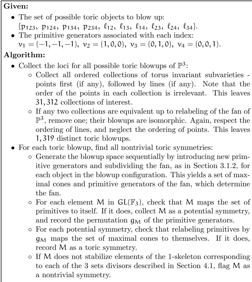
FIGURE 10. The computational technique by which we exhausted all possible toric symmetries of sequential toric blowups of \mathbb{P}^3
