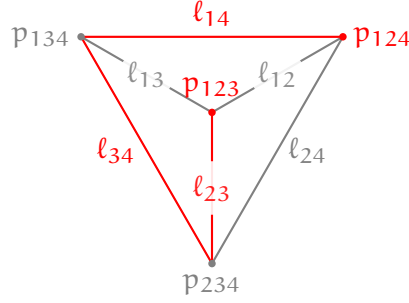
FIGURE 13. The torus-invariant subvarieties of \mathbb{P}^3 . The red subvarieties comprise the blowup locus for Class C, blown up in the following order: p_{124} , p_{123} , l_{34} , l_{23} , l_{14} .
