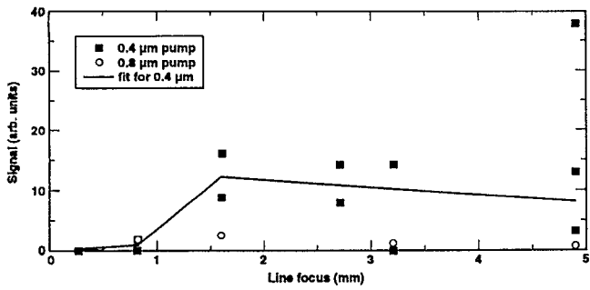
FIG. 3. The intensity versus length for the L_{\alpha} 135 Å transition in H-like Li for ionization of the ablated Li by the 100 fs Ti: Sapphire at 0.8 and 0.4 \mu\text{m} wavelengths.
