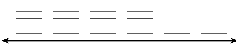
Figure 7. A linear (4, 15) -society with n = 21 voters. Here q = 4 and \rho = 2 , so the clique number is at least \lceil (n - \rho)/q \rceil = 5 .
