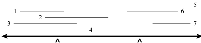
Figure 3. A linear society with a spectrum of two candidates (at platforms marked by carats): take the approval sets of the society of Figure 2 and intersect with these candidates. It is a (2, 4)-agreeable linear society.
