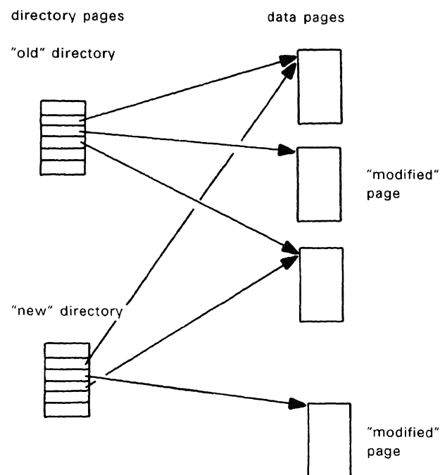
Figure 2-2: Sharing of pages through separate directories
