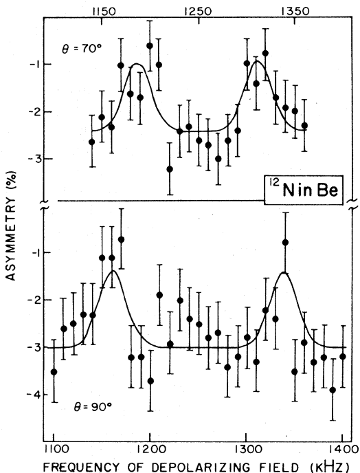
FIG. 1. Resonance scans of ^{12}\text{N} implanted in a single crystal of Be. \theta is the angle between the crystalline c axis and the applied magnetic field \vec{B} .
