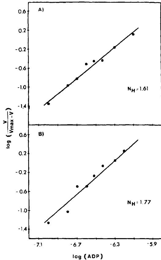
FIG. 3. Comparison of Hill plots for ADP-induced platelet shape change when V is measured by the light microscope method (A) and by the light transmission method (B). Data are taken from Fig. 1. In each case only the linear portion of the Hill plot has been shown. An analysis of covariance as described in Sokal and Rohlf (1969) was used to show that the slopes of these two Hill plots are not significantly different ( 0.5 > p > 0.25 ).
