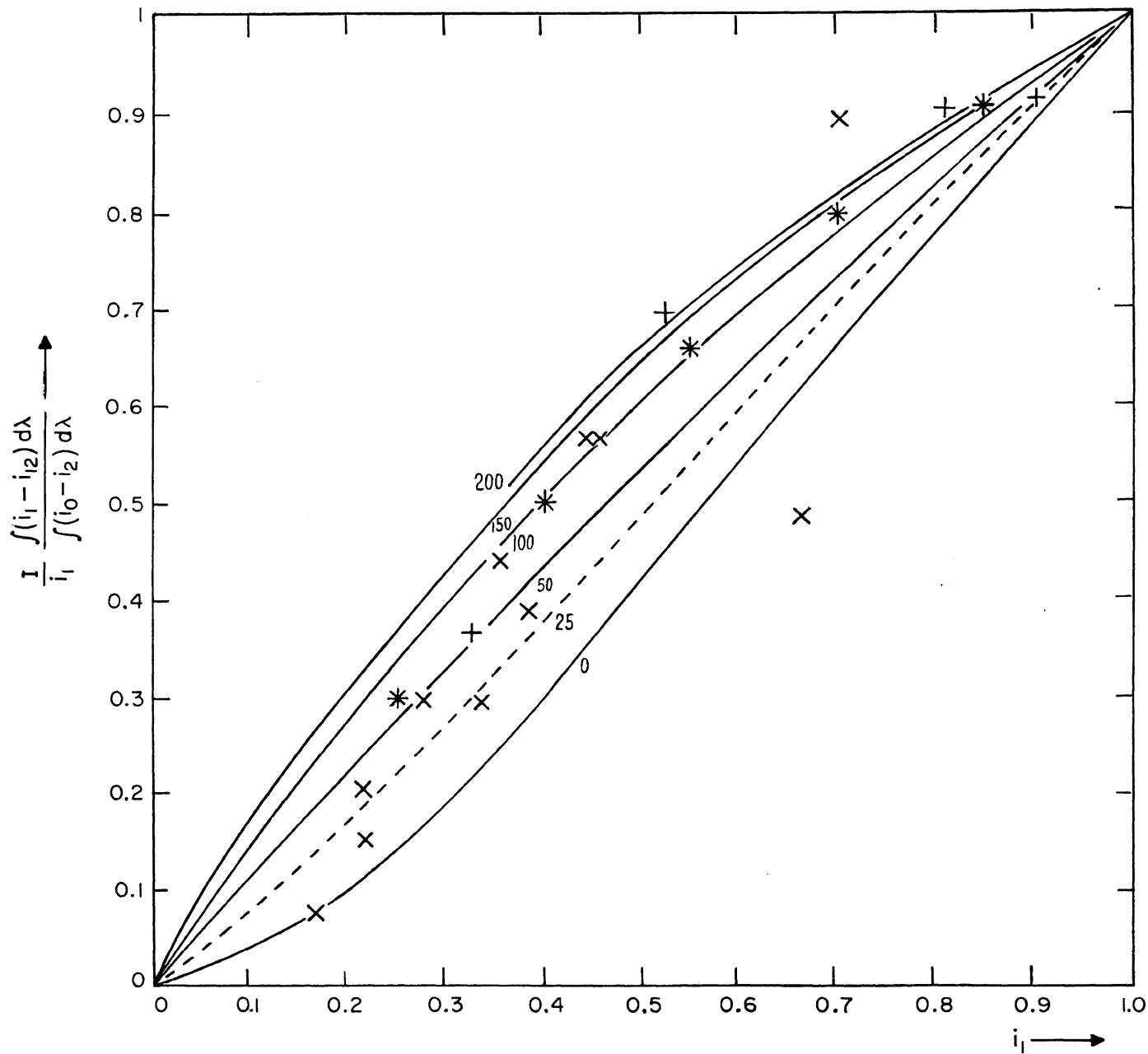
FIGURE 5. Influence of background on equivalent width.
