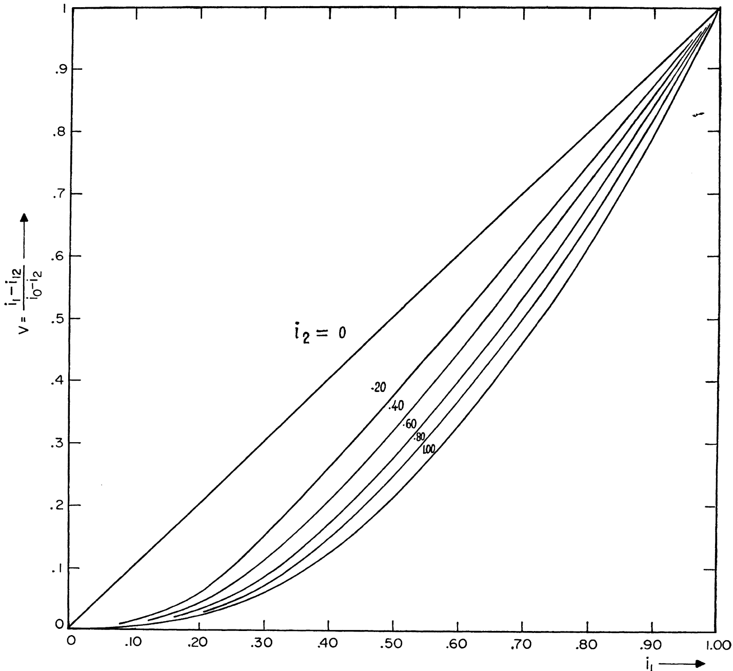
FIGURE 4. Monochromatic blend factor.
