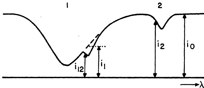
FIGURE 3. Disturbed and undisturbed Fraunhofer line.
