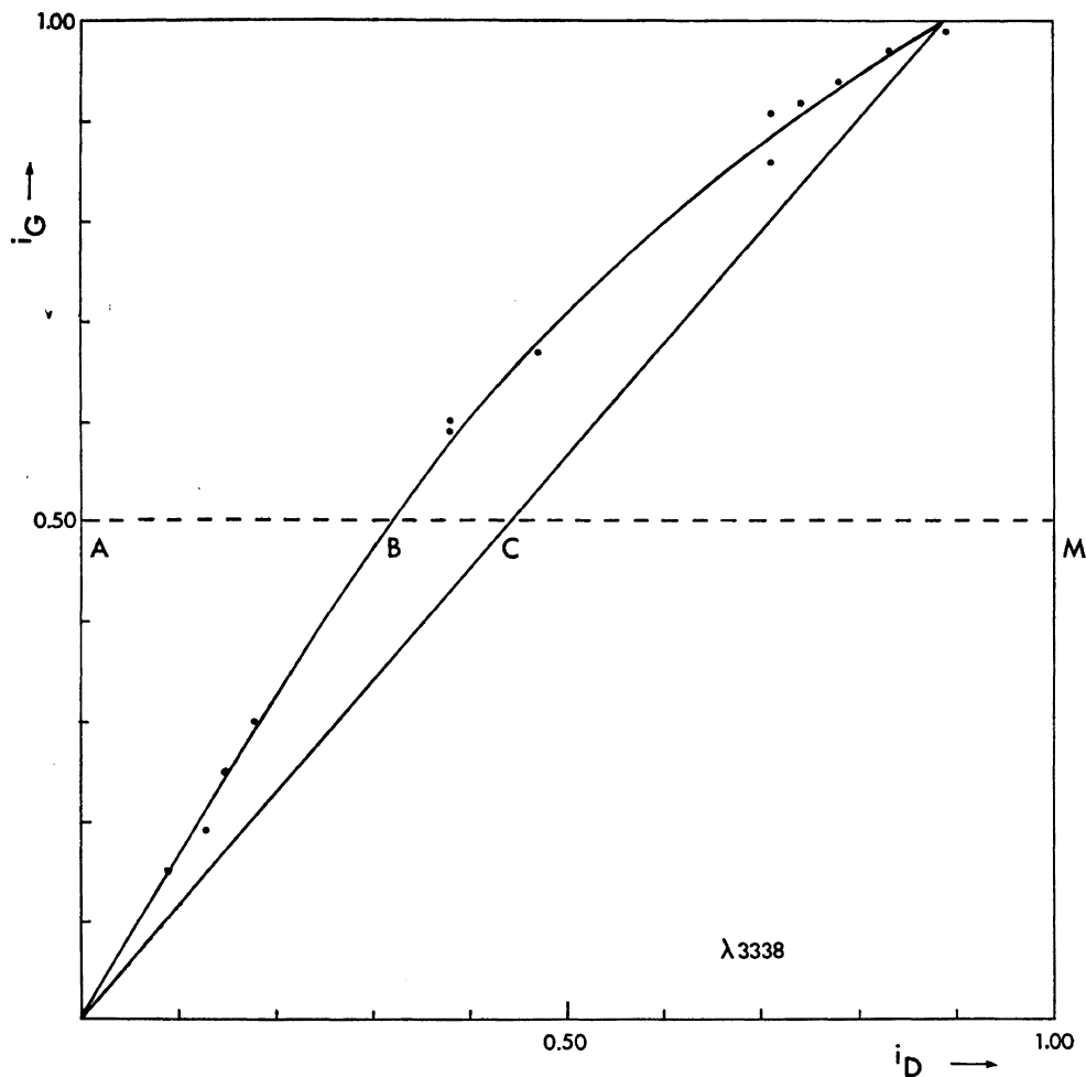
FIGURE 2. Comparison of UV monochromatic intensity measurements at Göttingen and at Dunsink. Coordinates i_G and i_D in arbitrary units.
