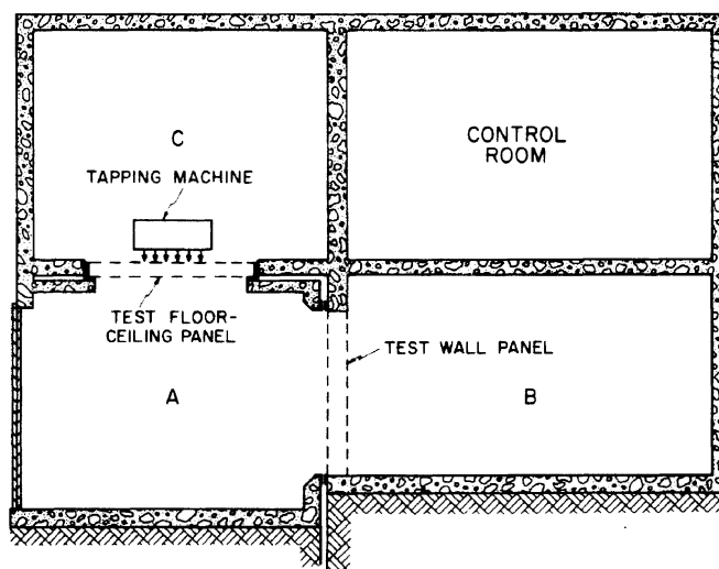
FIGURE 1. Vertical section of NBS sound transmission facilities.
