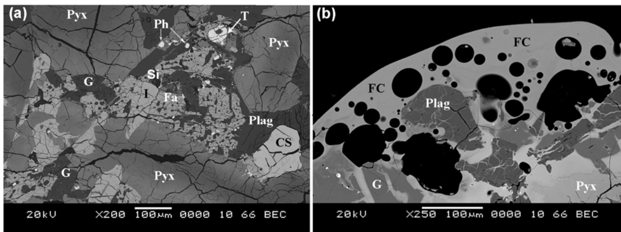
Fig. 11. (a) Back scattered electron (BSE) image of a mesostasis area in LAP 02205. Bleb like glass pockets are enclosed by fayalite groundmass and larger glass-rich regions. Mesostasis products enclosed by Fe-rich pyroxenes, ilmenites and plagioclase crystals. (b) BSE image of the fusion crust of LAP 02224. The vesicular grey area at top of section is the fusion crust – minerals being melted into this zone can be seen at the bottom of this zone. Vesicles (black circular regions) are heterogeneously distributed throughout the melted/melting area. Dark grey minerals are plagioclases; pale grey at the base of the image are pyroxenes; small bright white blebs are troilite. Minerals are represented by the same symbols in Figure 9 and Fa=fayalite, T=Troilite Fa=fayalite groundmass, G=Glass, Ph = Phosphates, FC = Fusion Crust
