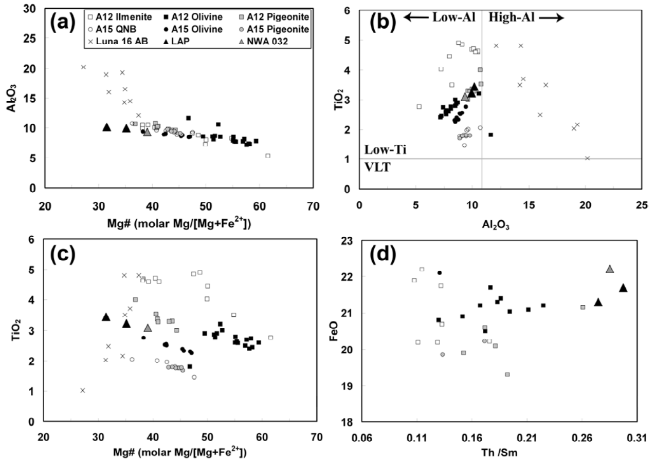
Fig.12. Bulk composition variation diagrams comparing LAP to low-Ti basalts from the A12, A15 and Luna 16 collection. Apollo compositions are taken from Rhodes and Hubbard (1973), Rhodes et al. (1977), BVSP (1981), Neal et al. (1994a), and average bulk composition data for NWA 032 are taken from Zeigler et al. (2005). (a) LAP has the lowest Mg\# of the low-Al, low-Ti basalts; (b) a plot of TiO_2 against Al_2O_3 shows that the LAP stones are all within the low-Ti, low-Al lunar mare basalt classification as proposed by Neal and Taylor (1992); (c) TiO_2 and Mg\# are good distinguishing characteristics for the Apollo basalts – the different olivine, pigeonite, ilmenite and QNB basalts all fall into distinctive groupings, with the LAP stones not easily being fitted into any group; (d) LAP, along with NWA, is highly enriched Th (and other ITEs) compared to the other basalts.
