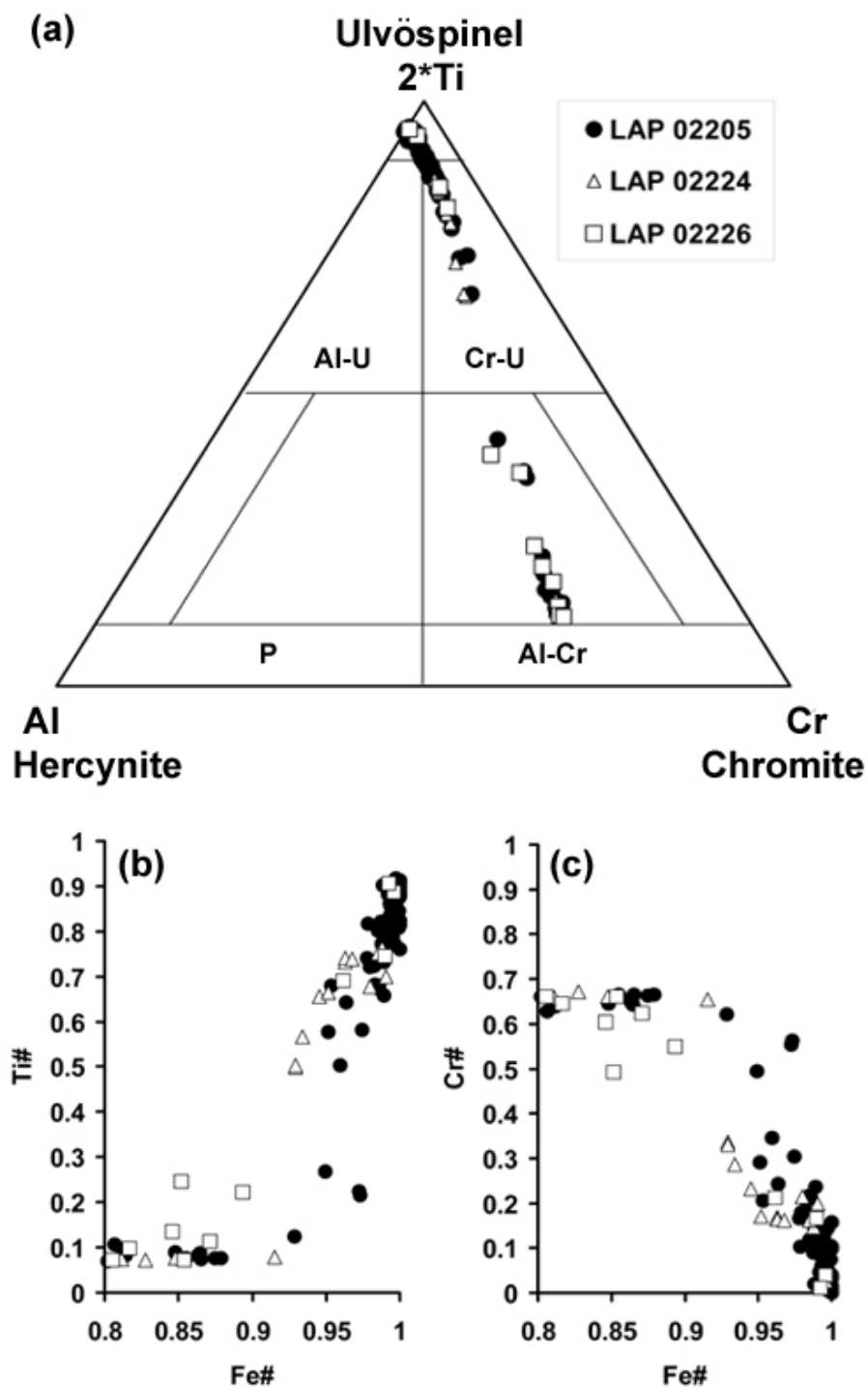
Fig.10. (a) Compositional diagram (2Ti-Cr-Al in mol %) for spinels analyzed in LAP 02205, LAP 02224 and LAP 02226. Compositions zones: P = picotite, Al-Cr = aluminous chromite, Al-U = aluminous ulvöspinel, Cr-U = chromian ulvöspinel. (b) Plot of Fe# (molar \text{Fe}^{2+} / [\text{Fe}^{2+} + \text{Mg}] ) vs. Ti# (molar \text{Ti} / [\text{Fe}^{2+} + \text{Mg}] ).
