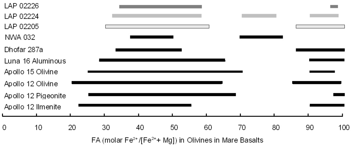
Fig. 8. Comparison of olivine Fe# (molar Fe/ [Fe + Mg]) compositions in LAP 02205, LAP 02224 and LAP 02226 compared to mare basalt olivine compositions (Pakike et al. 1991) and basaltic lunar meteorite Dhofar 287a (Anand et al. 2003b) and NWA 032 (Anand et al 2006). LAP lunar stones show a similar range to Apollo 12 and 15 basalts, albeit with a higher Fe# value for the most primitive forsterites. LAP 02224 shows an intermediate range of olivine chemistries which correspond to the Fe-rich rims of large olivine crystals.
