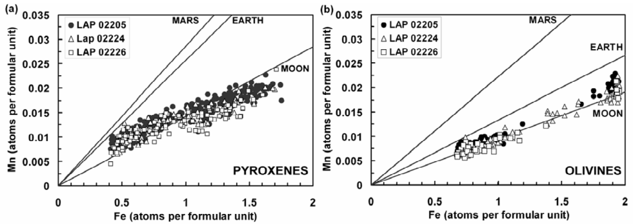
Fig.2. Fe to Mn ratios in pyroxenes and olivines are an indicator of planetary origin as lunar pyroxenes and olivines exhibit diagnostic Fe/Mn ratios compared to the Earth, Mars, Vesta and chondrites, probably as the result of volatile loss in an early Moon-forming event (Papike et al. 2003). Fe-Mn ratios in LAP 02205, 02224 and 02226 (Tables 2 and 3) for (a) pyroxenes and (b) olivines compared to typical planetary fractionation trends compiled by Papike et al. (2003). Atoms per formula unit are based on 4 oxygen atoms for olivine and 6 oxygens for pyroxene.
