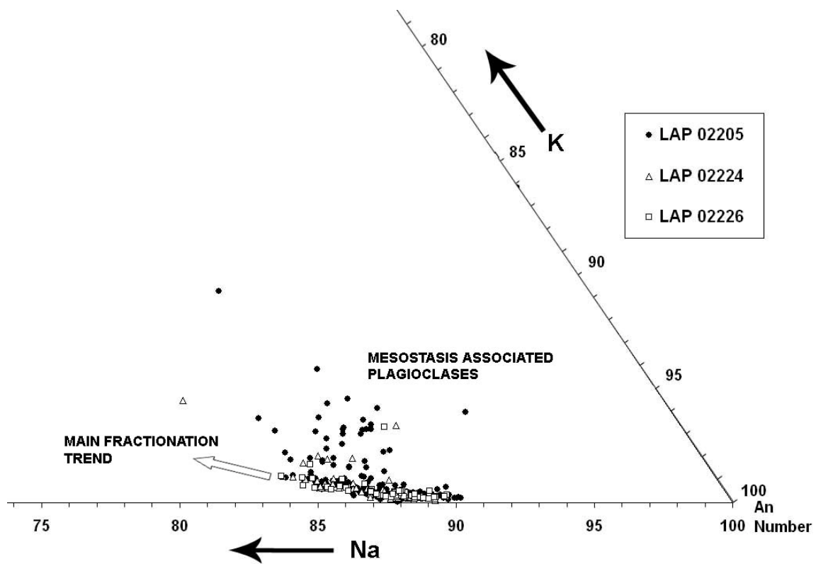
Fig. 7. Ternary plot of plagioclase content in LAP 02205, 32, LAP 02224, 35 and LAP 02226, 25 showing typical trend of basalt fractionation (increasing Or and Abs-content with decreasing An-content). K-enriched compositions that exhibit a scattered trend representing those plagioclase grains associated with mesostasis areas.
