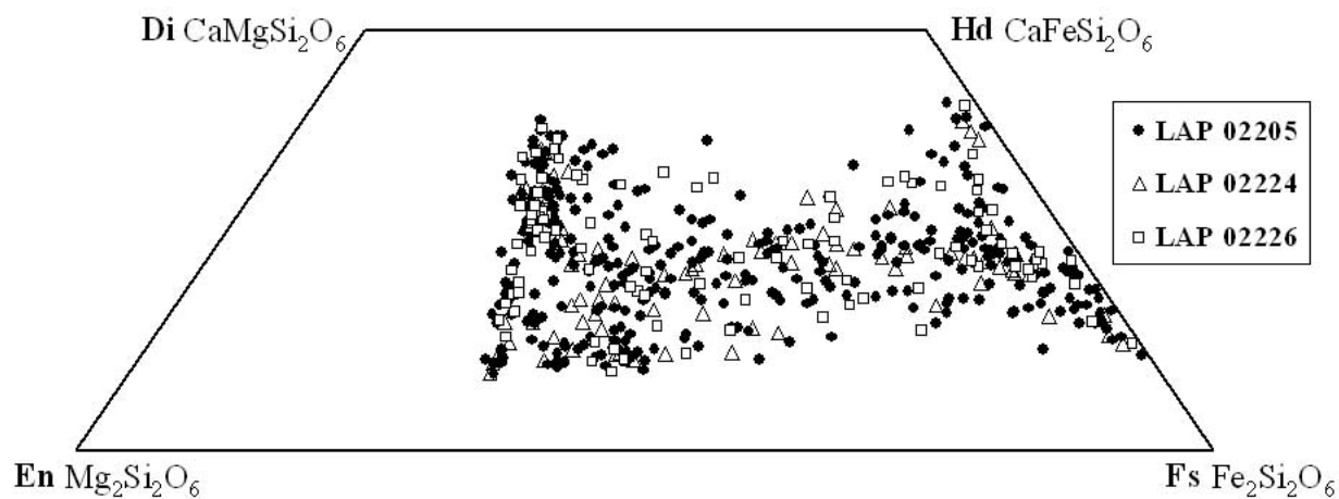
Fig. 4. Pyroxene compositions in LAP 02205, 32, LAP 02224, 35 and LAP 02226, 25 plotted on a pyroxene quadrilateral. The three stones show very similar compositional trends with pyroxenes zoned from Mg-rich cores to Fe-rich rims. This similarity is evidence that the stones are geochemically related and are likely to have originated from the same lava flow.
