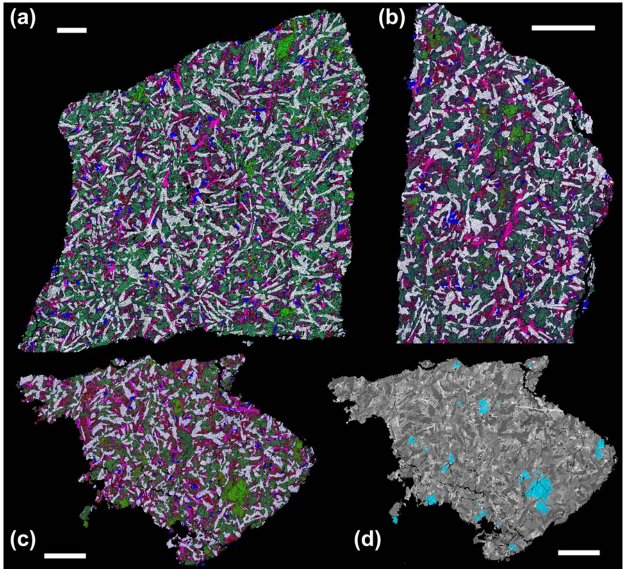
Fig. 3. False color X-ray maps of sections of (a) LAP 02205,32, (b) LAP 02224,35, and (c) LAP 02226,25 where white represents Al (plagioclases), yellow represents Ca (plagioclase), red represents Fe (pyroxene rims and fayalitic areas), green represents Mg (pyroxene cores and forsteritic olivines), blue represents Si (cristobalite grains), and pink represents Ti (ilmenite and spinel) enriched areas. This technique particularly highlights the location of forsteritic olivine (bright green areas), fayalite (brightest red areas), ilmenite (pink), silica (blue) and plagioclase (white phases). (d) The locations of forsteritic olivine are highlighted on a montaged back-scattered electron image of thin section LAP 02226,25 - similar phase maps were compiled for all other mineral phases. The proportional number of pixels from each identified phase is then used to calculate a mineral mode for the section (Table 5). Scale bars are 1 mm.
