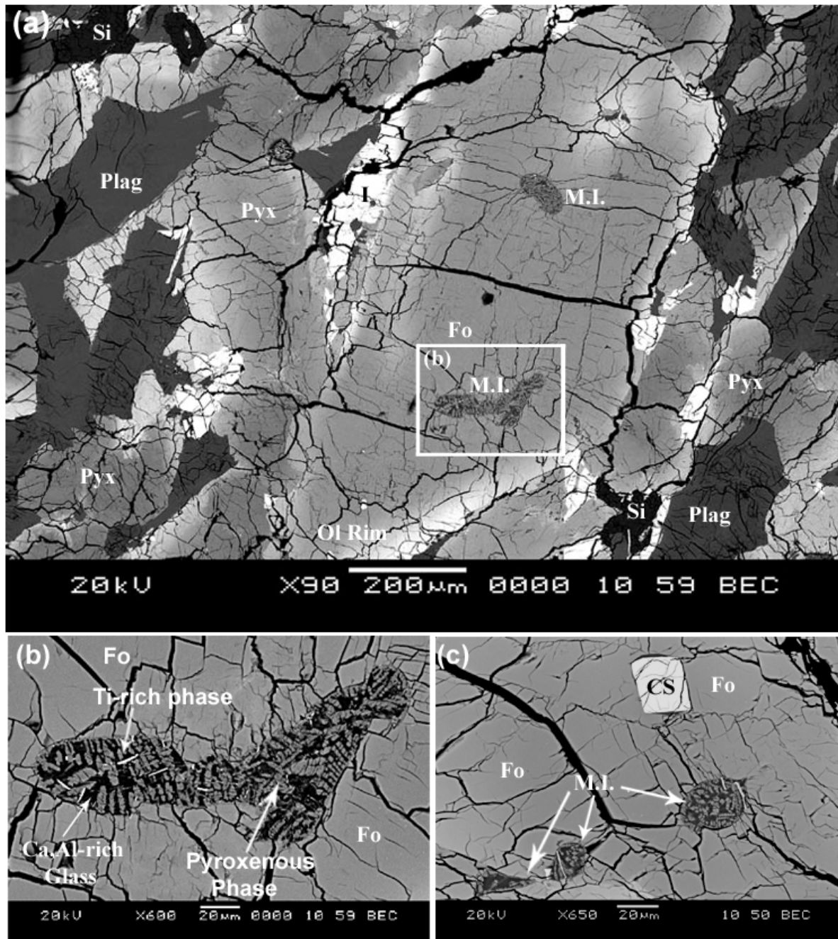
Fig. 9 (a) BSE image of large olivine grain in LAP 02205. The mineral is zoned from Fo 63 core to Fo 39 rims and contains two small quenched melt areas which have been highlighted. (b) Close-up of the trapped melt with microcrystalline texture in LAP 02205 where daughter barred pyroxene microcrysts sit in a glassy matrix with micro inclusions of a Ti-rich and small S-rich phases (bright albedo). (c) Close-up of small trapped melt inclusions in a single olivine in LAP 02224. Minerals are represented by the following symbols: Pyx=pyroxene; Plag=plagioclase; I=ilmenite; Fo= Forsteritic olivine; CS= chromite-spinel; MI = Melt Inclusion; Si=silica; Ol Rim=olivine rim.
