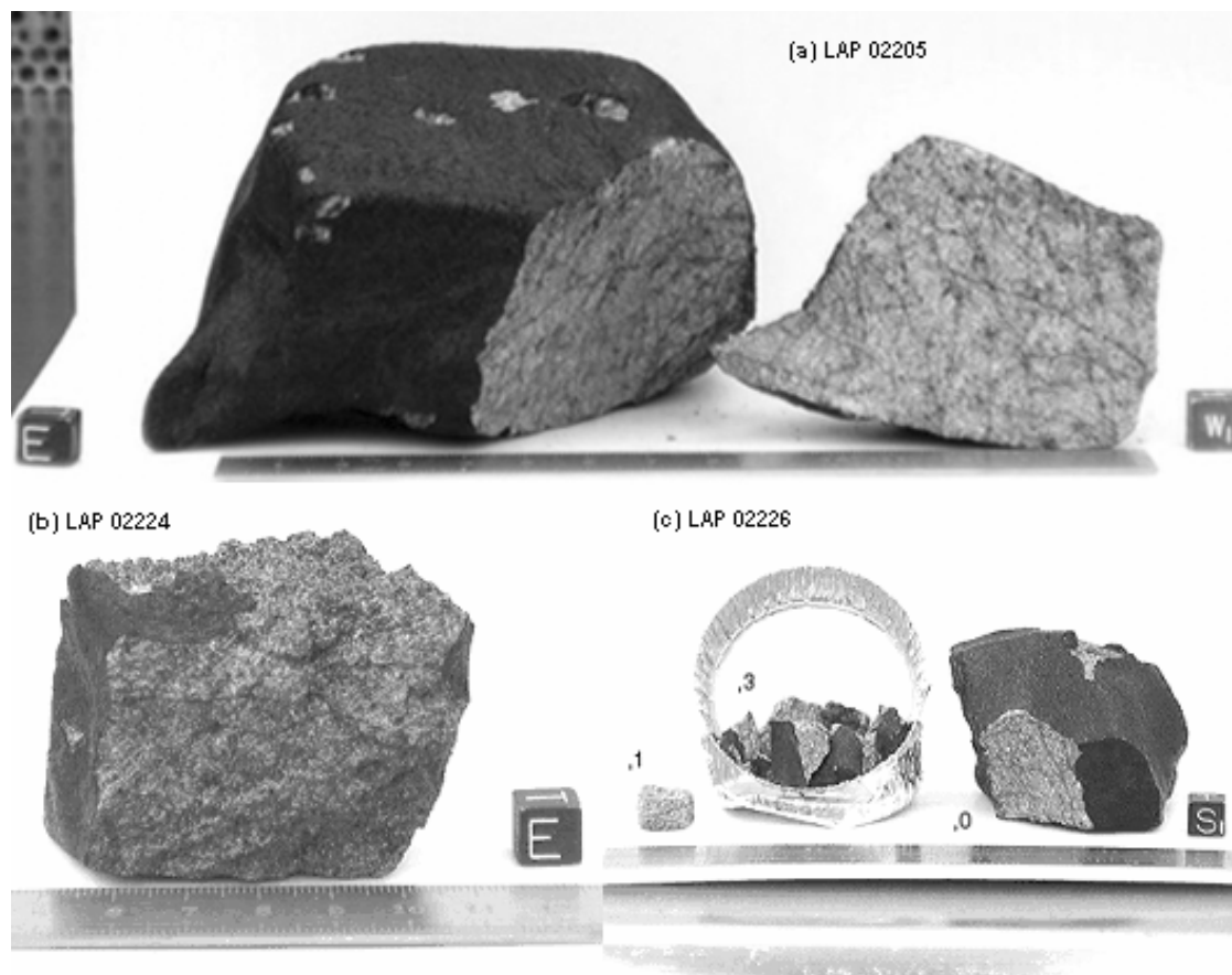
Fig. 1. Photographs of (a) LAP 02205, (b) LAP 02224, and (c) LAP 02226 stones in hand specimen. All three stones have a dark brown/black fusion crust. The scale cube is 1 cm on a side. Photographs courtesy of Scatterwaite (2003, 2004a).
