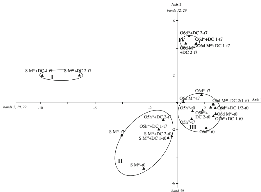
Fig. 3 PCA biplot of DGGE band patterns from microcosm assays. The bands of culture DC members were excluded in the bioaugmentation patterns
