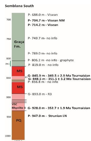
Fig. 1 – Simplified stratigraphic log of the studied Semblana PSN44 drillhole (Lunding Mining) (after Pereira et al., 2014); P - sample for palynostratigraphical study; G - sample for zircon geochronology. Graça Fm. (Upper Visean); MS – massive sulphide, VSC – felsic volcanics (rhyolite), PQ – Phyllite-Quartzite Fm (Strunian-Famennian). Bold lines – thrust faults.
