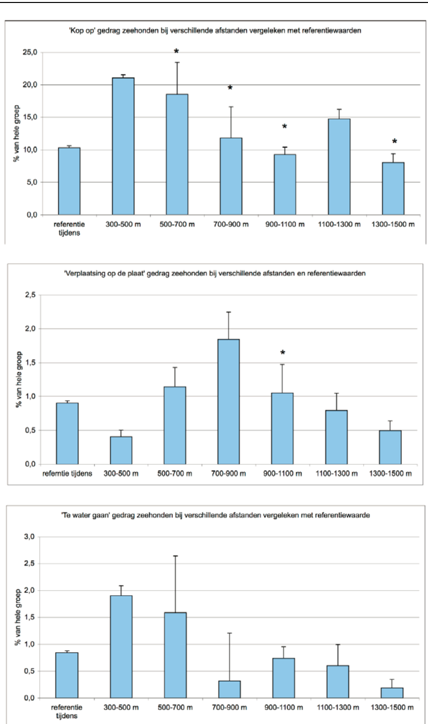
Figure 17.6. The reaction of seals on an approaching TSHD.
