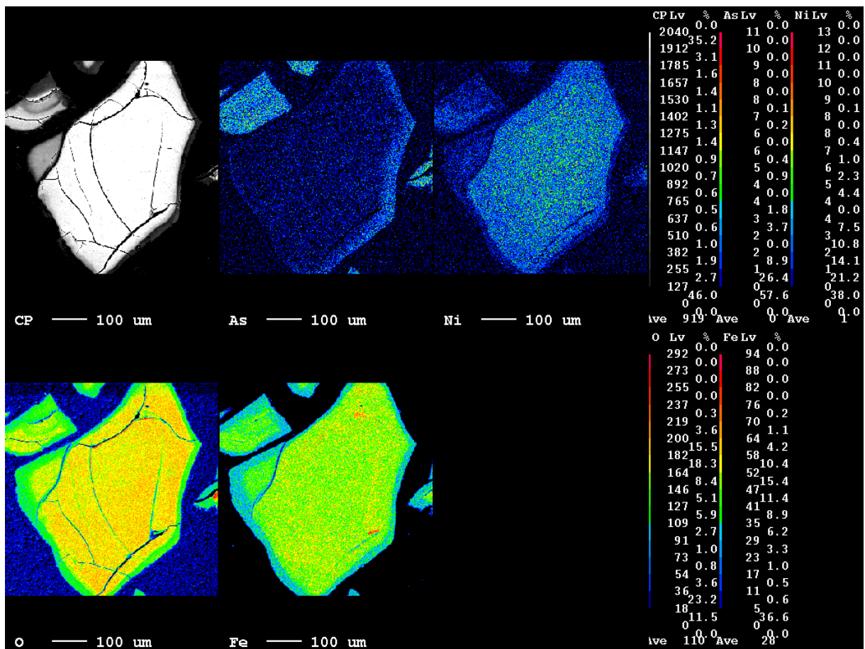
Figure 6 – Mapping of concentration of different elements in a Particle of ARM 300
