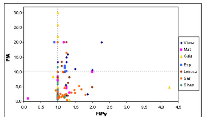
Figure 11. Phenanthrene and anthracene concentration rates (P/A) and fluoranthene and pyrene rates (FI/Py) for all sampling sites in 2002-2004.
