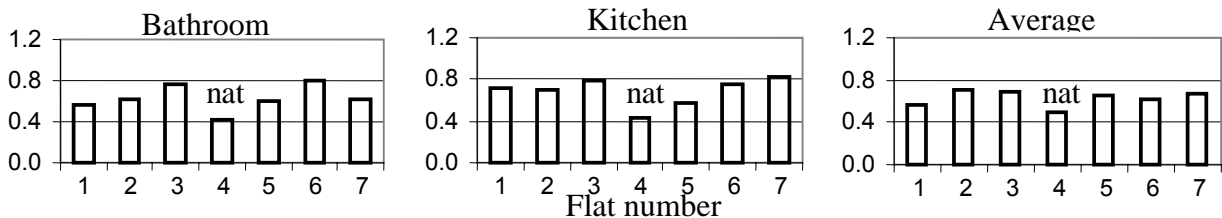
Figure 3: Display of measured ACH during the summer conditions 2/8-9/8
