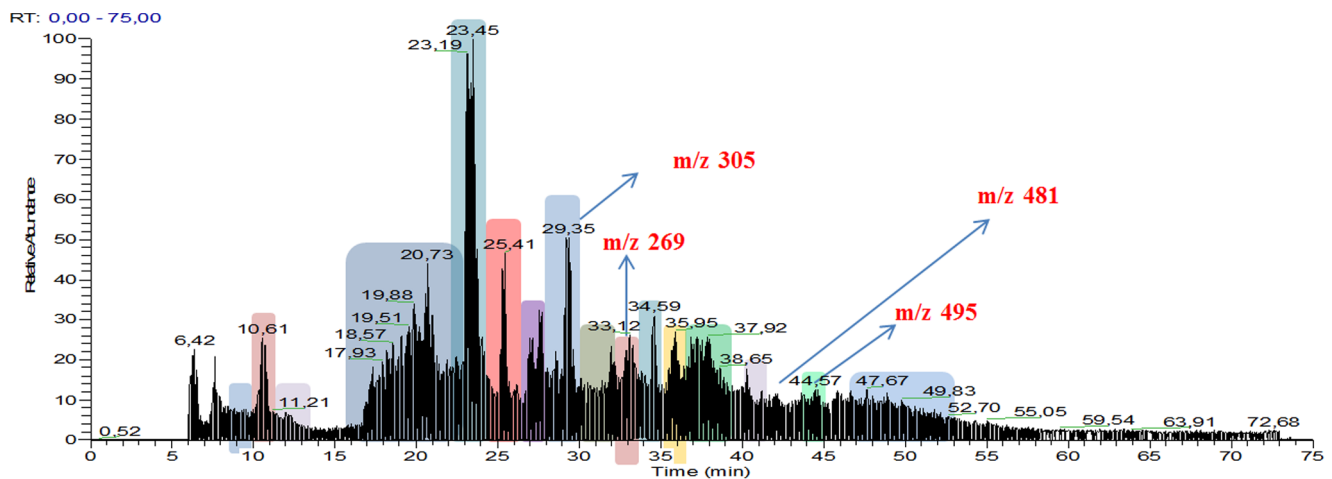
Figure 3. Typical spectra of representative estrogen metabolites, which were obtained in a single injection. The m/z of the molecules and the respective retention time at which they appear are highlighted.
