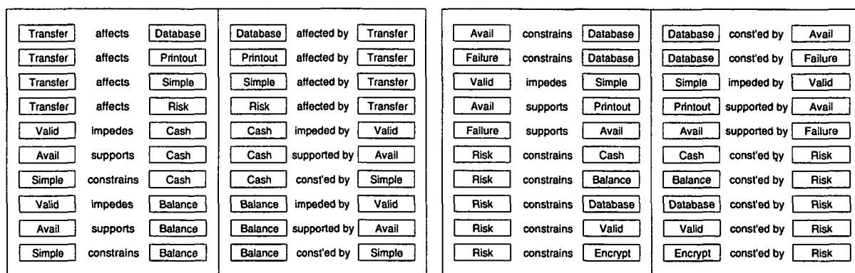
Fig. 4 Pre-recorded traceability relationships
