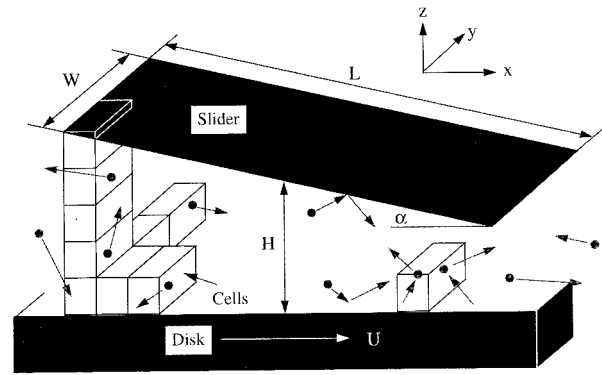
FIG. 1. DSMC System Configuration.
