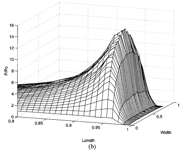
FIG. 8. Pressure profile for Kn = \infty ( H_{\min} = 0 nm): (a) side view and (b) 3-D view.
